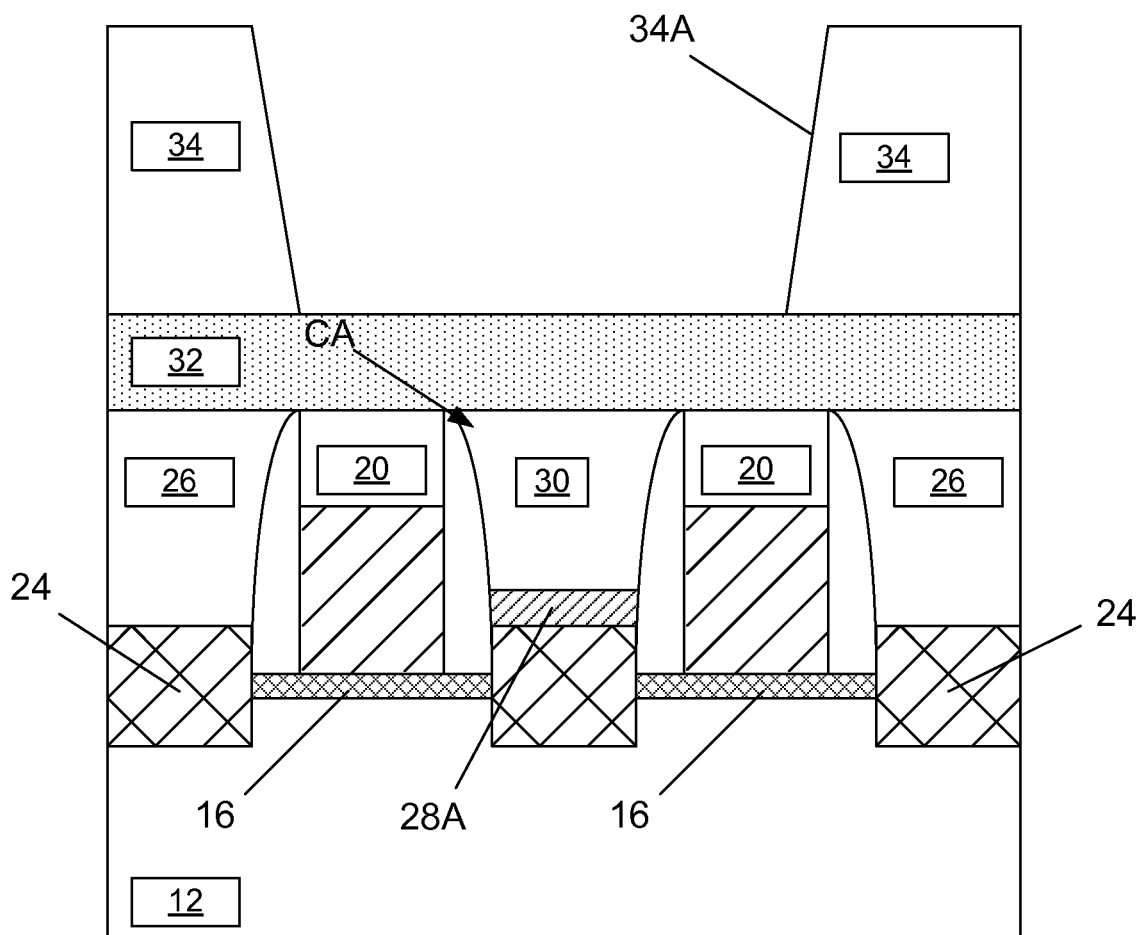
Figure 1D (Prior Art)
