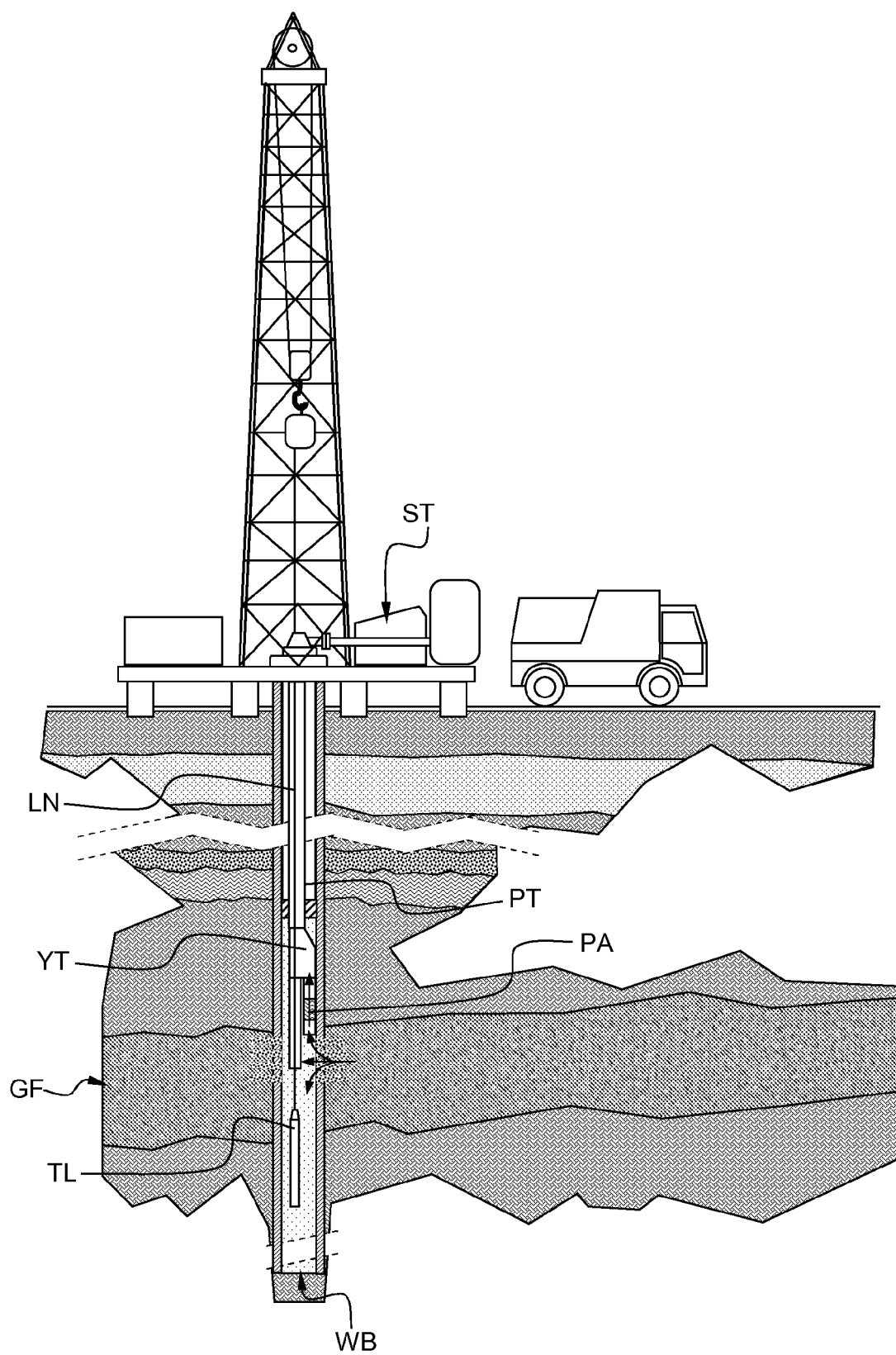
FIG. 1 - PRIOR ART
