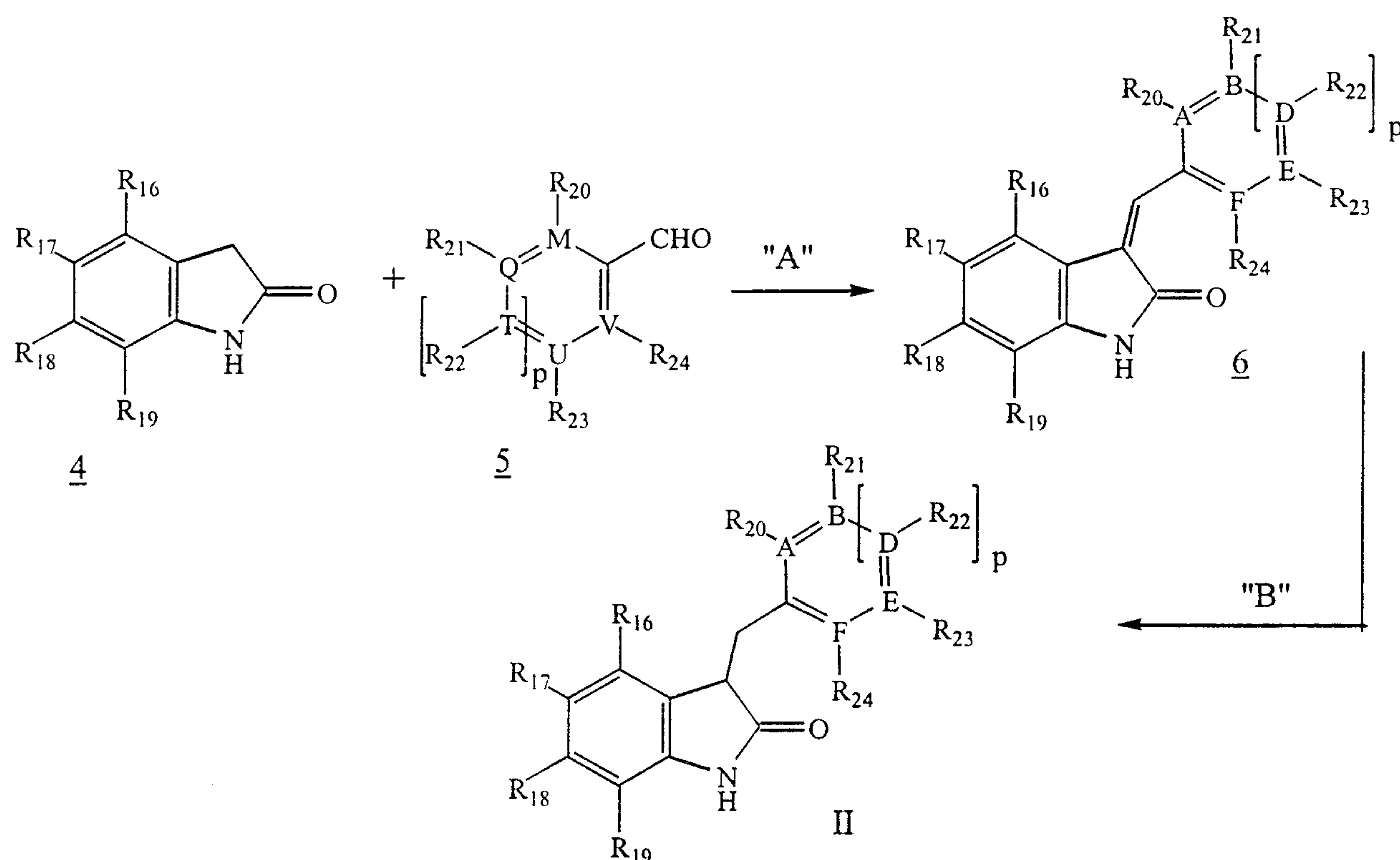
SCHEME II
