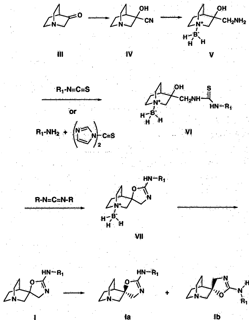
Scheme 1.
