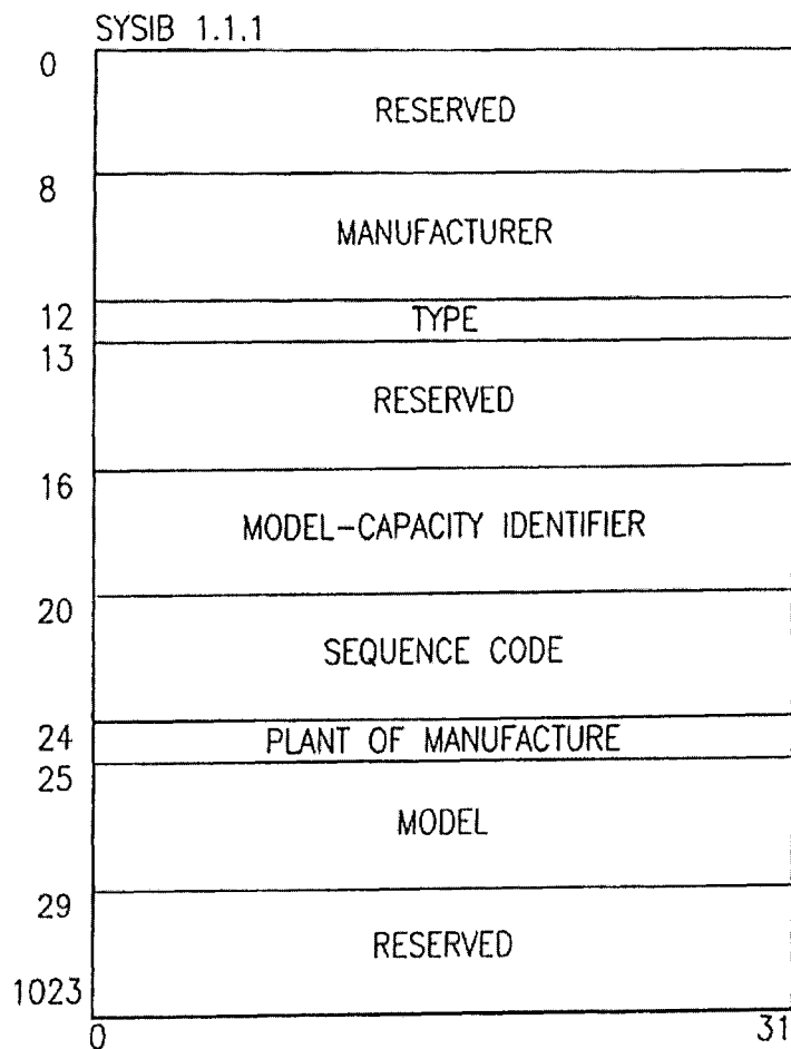
FIG.6 Prior Art
