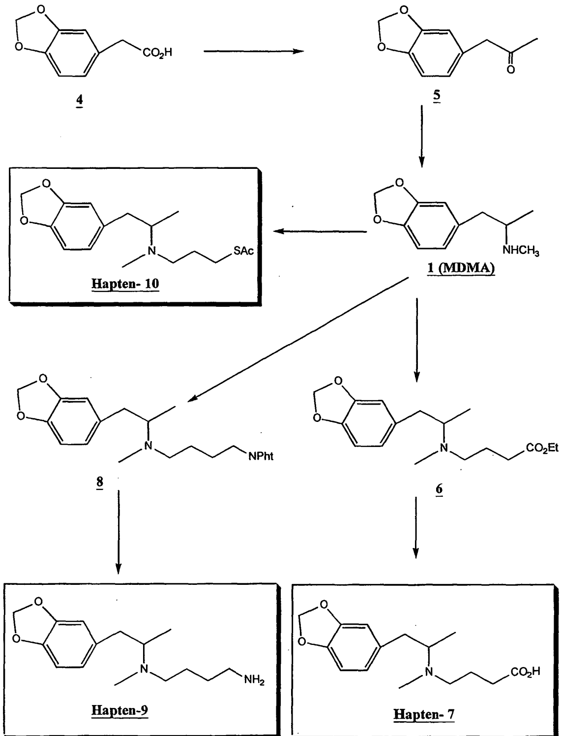
Figure -1: Chemical reaction for the preparation of haptens 7, 9 and 10
