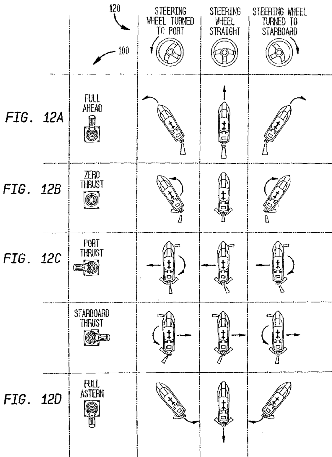
SINGLE WATERJET MOTION DIAGRAM
