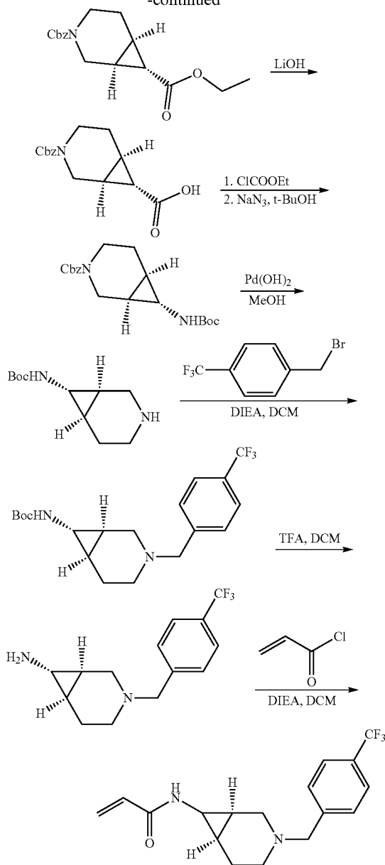
Step 1: 04-Benzyl 07-ethyl (1R,6S,7S)-4-azabicyclo[4.1.0]heptane-4,7-dicarboxylate
