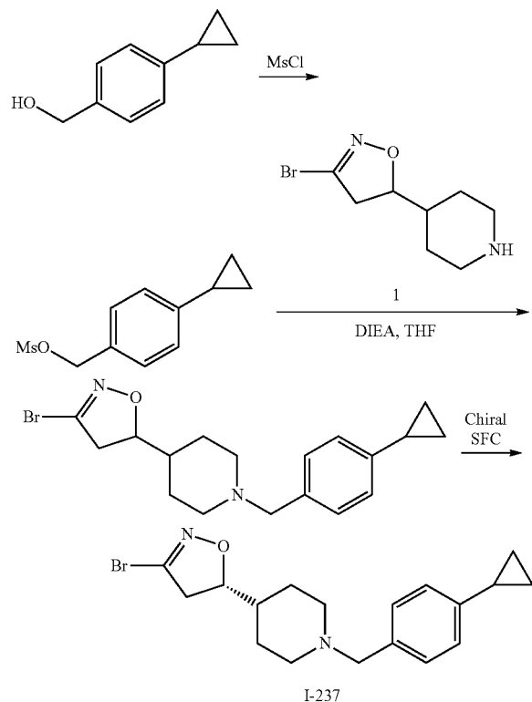
Step 1: (4-Cyclopropylphenyl)methyl methanesulfonate
