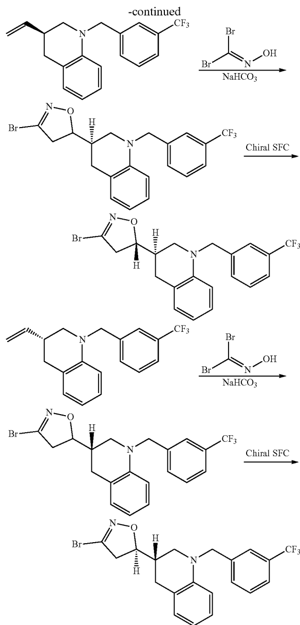
Step 1: Methyl quinoline-3-carboxylate
