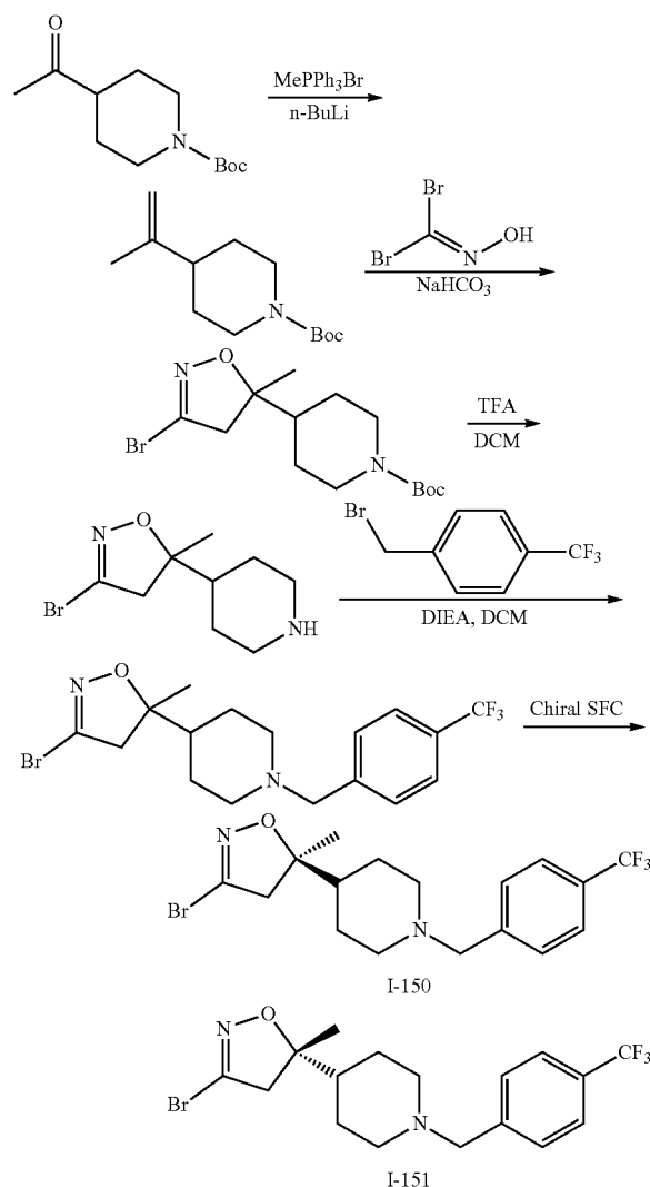
Step 1: tert-Butyl 4-isopropenylpiperidine-1-carboxylate
