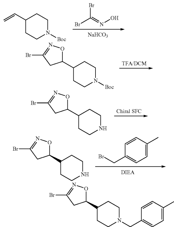
Step 1: tert-Butyl 4-(3-bromo-4,5-dihydroisoxazol-5-yl)piperidine-1-carboxylate
