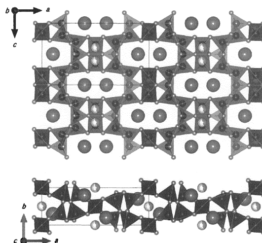
Crystal structure of \text{Li}_1\text{Ba}_2\text{Al}_1\text{Si}_7\text{N}_{12}
