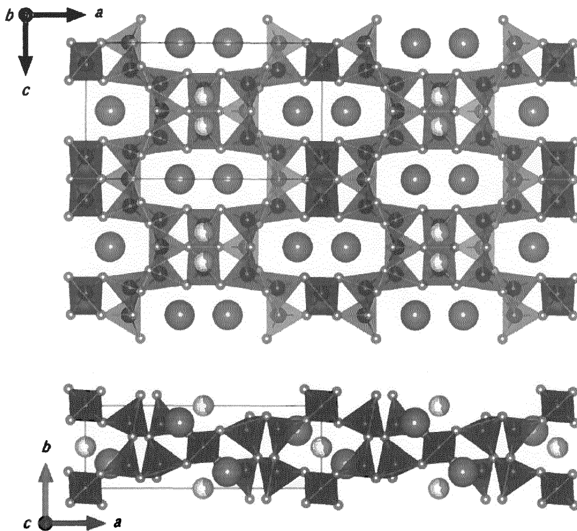
Crystal structure of \text{Li}_1\text{Ba}_2\text{Al}_1\text{Si}_7\text{N}_{12}
