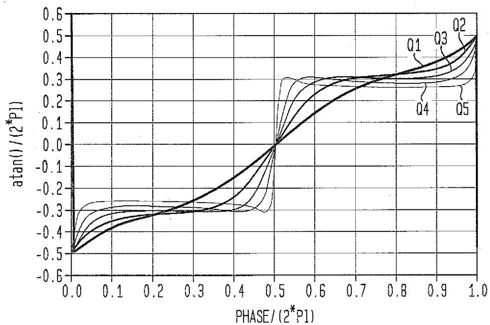
FIG. 5B CONTROL RESPONSE
