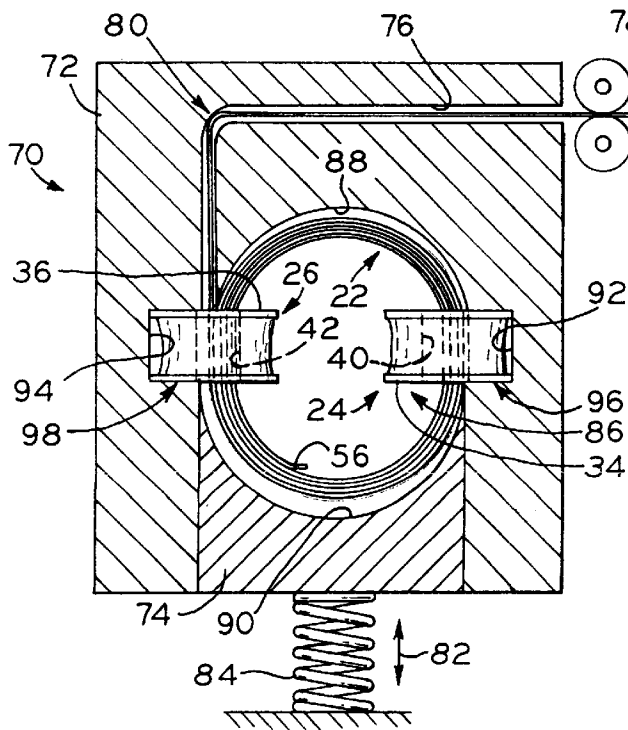
FIG. 1C PRIOR ART
