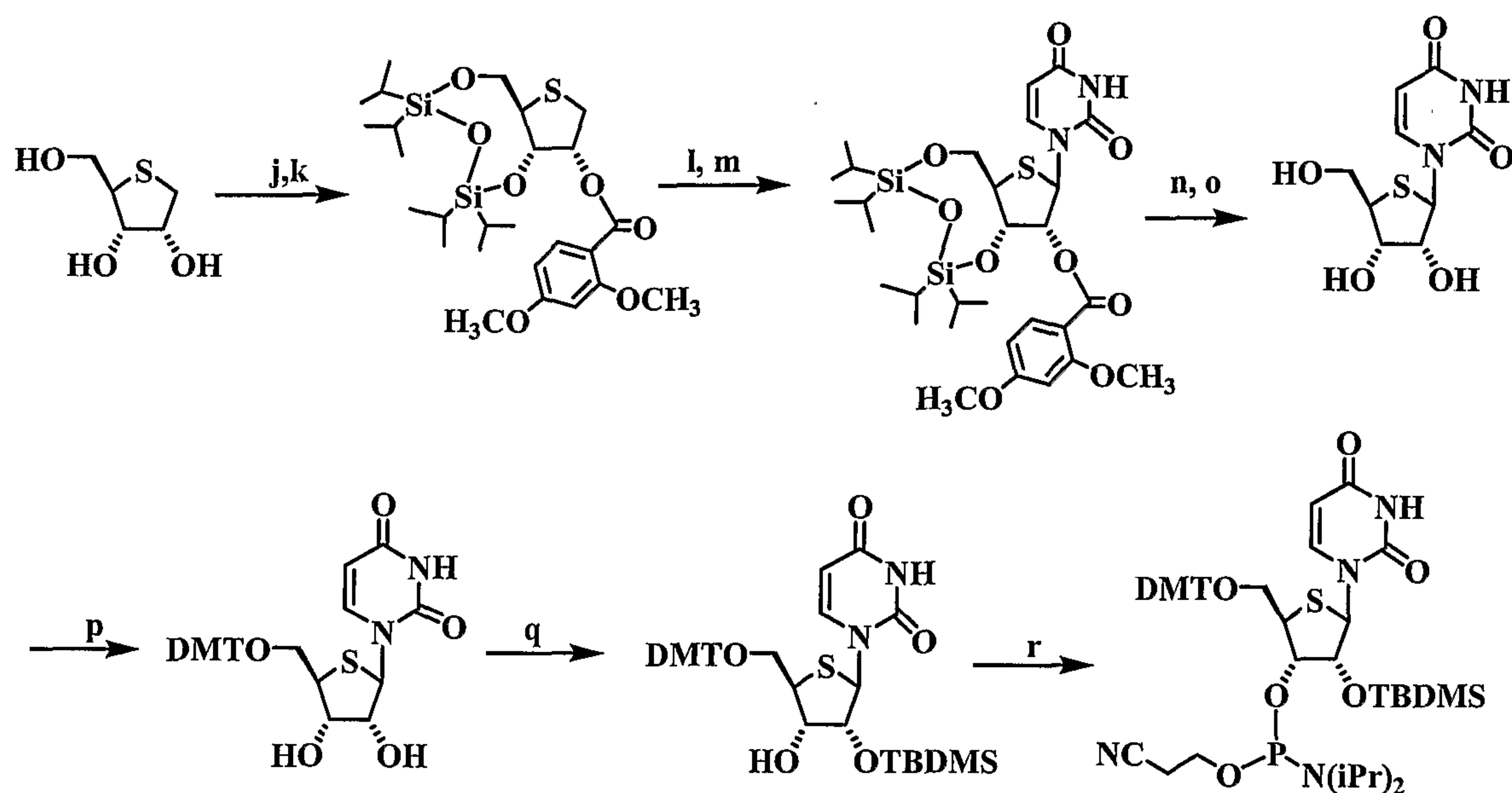
Scheme 3 : Synthesis of 4'Thio-U Phosphoramidite
