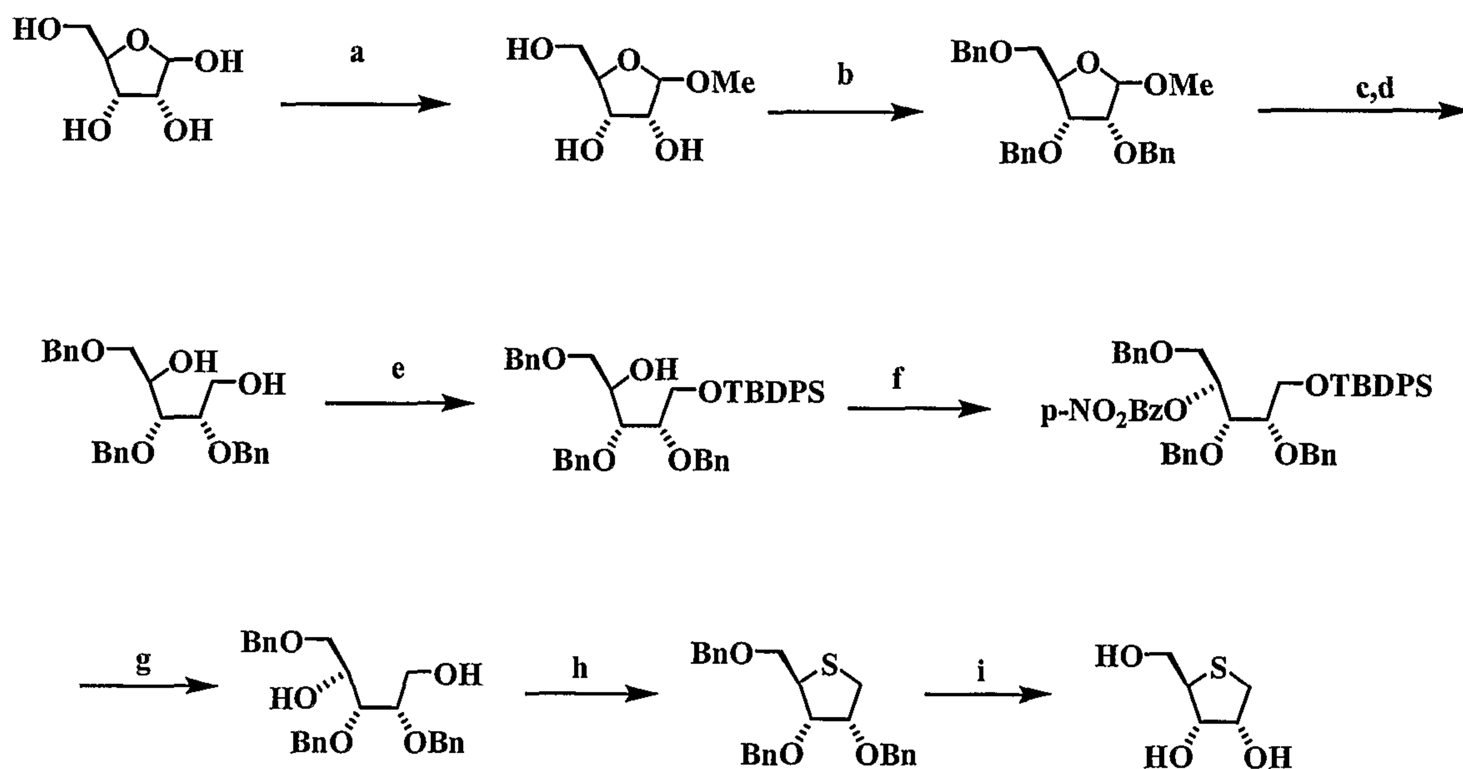
Scheme 2: Synthesis of a thio-sugar
