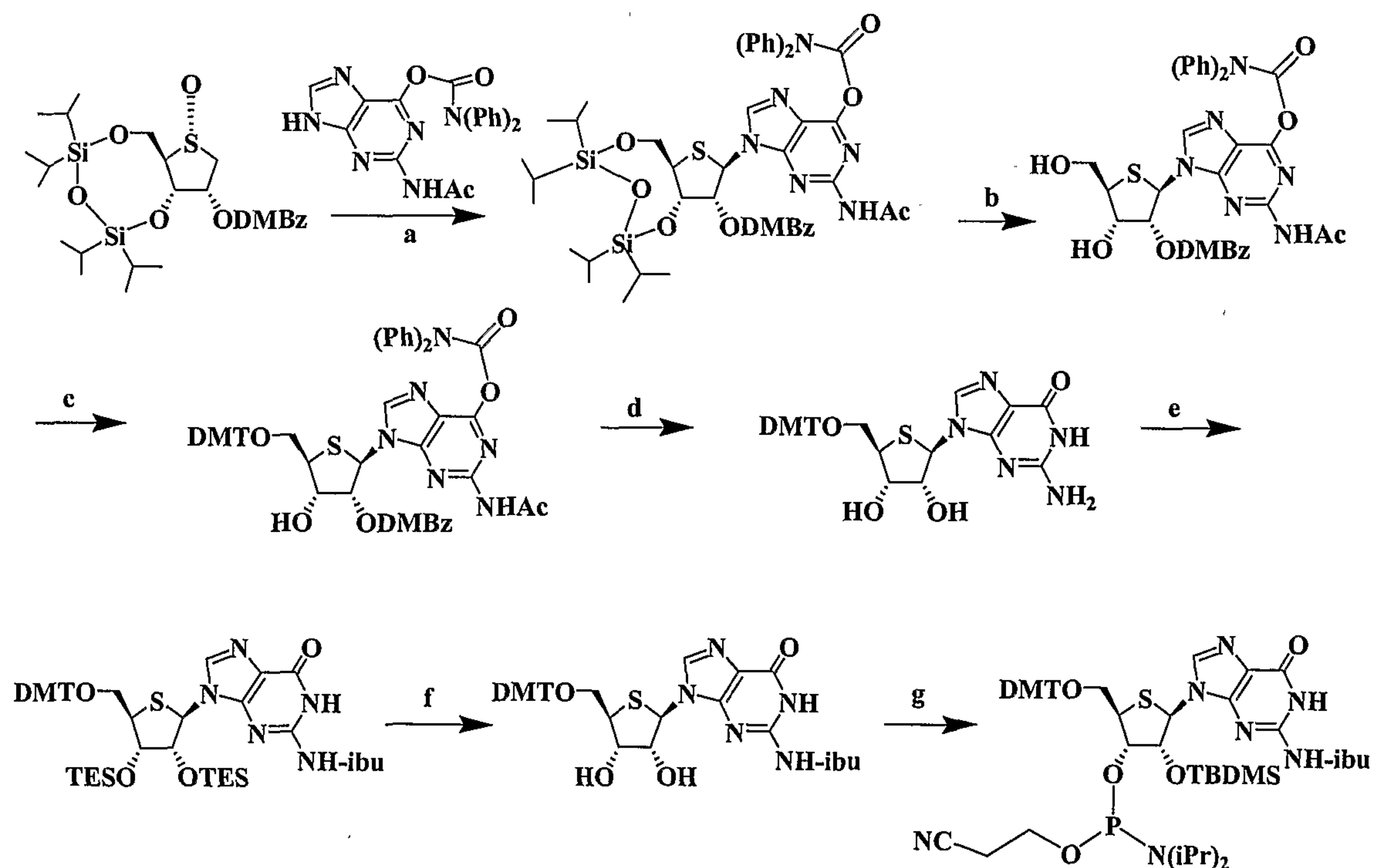
Scheme 5: Synthesis of 4'-Thio-G Phosphoramidite
