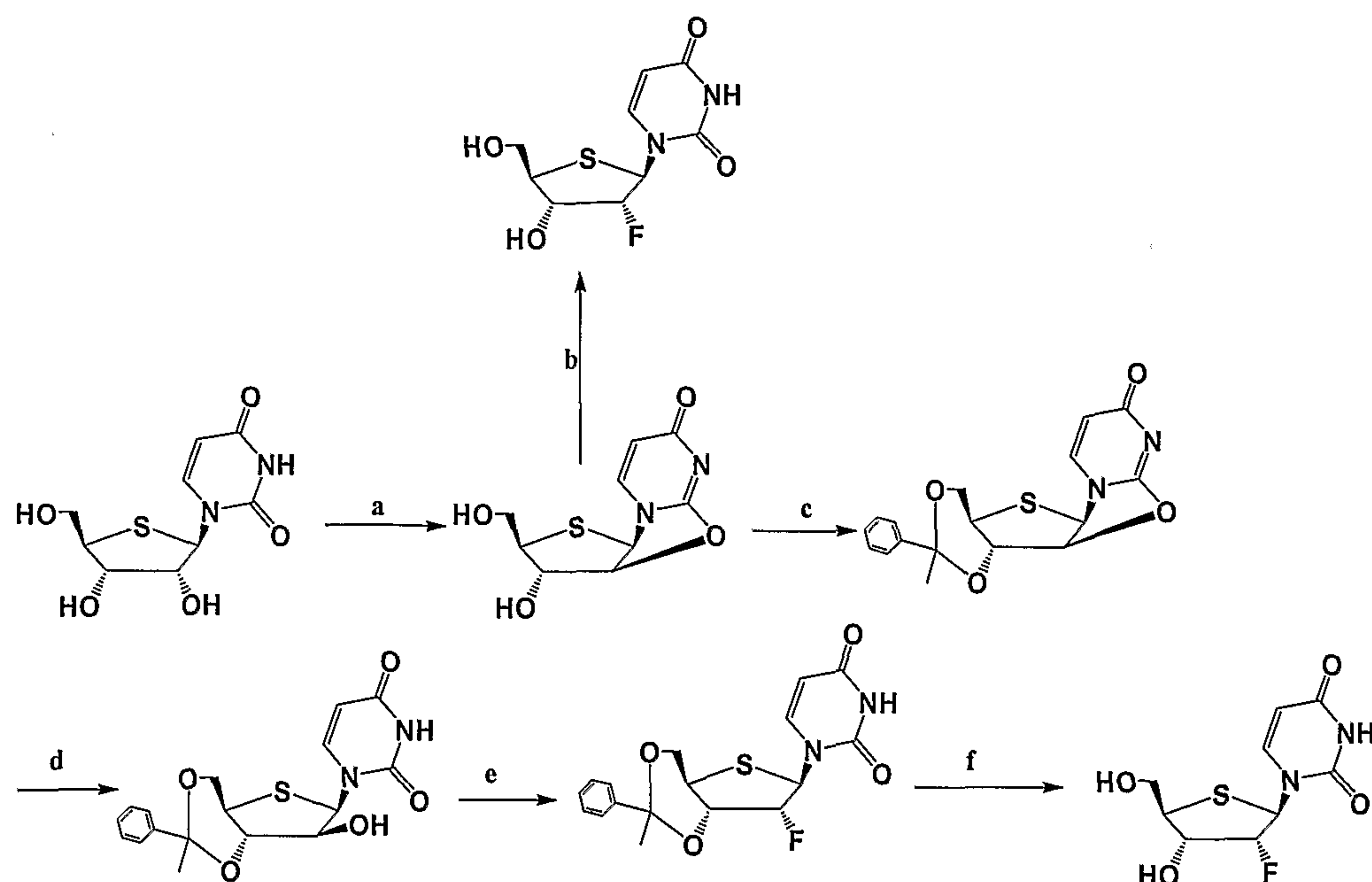
Scheme 8: Synthesis of 2'-fluoro-4'-thio-uracil
