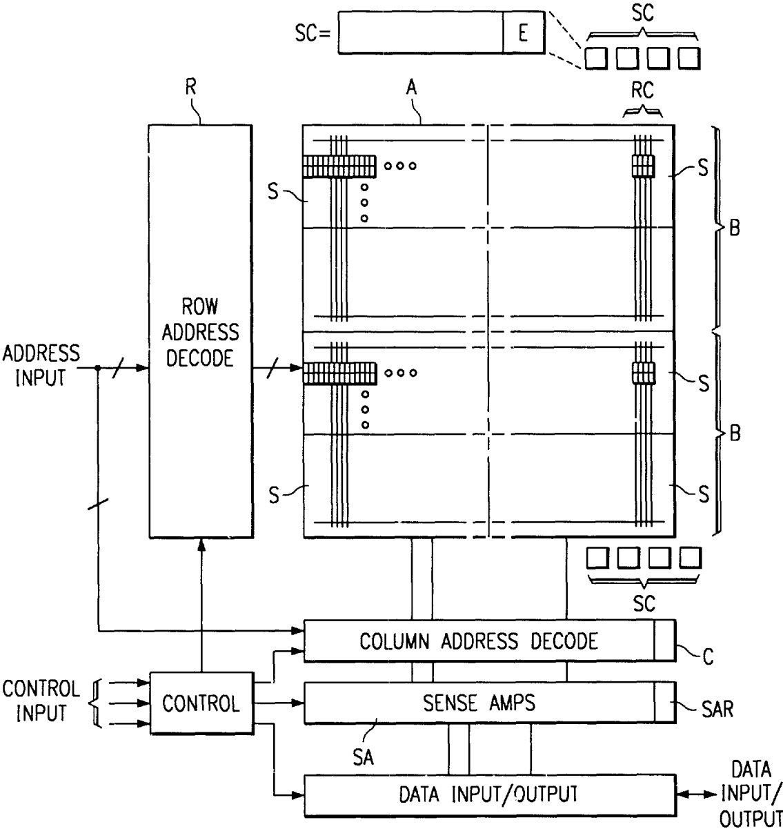
FIG. 1 (PRIOR ART)
