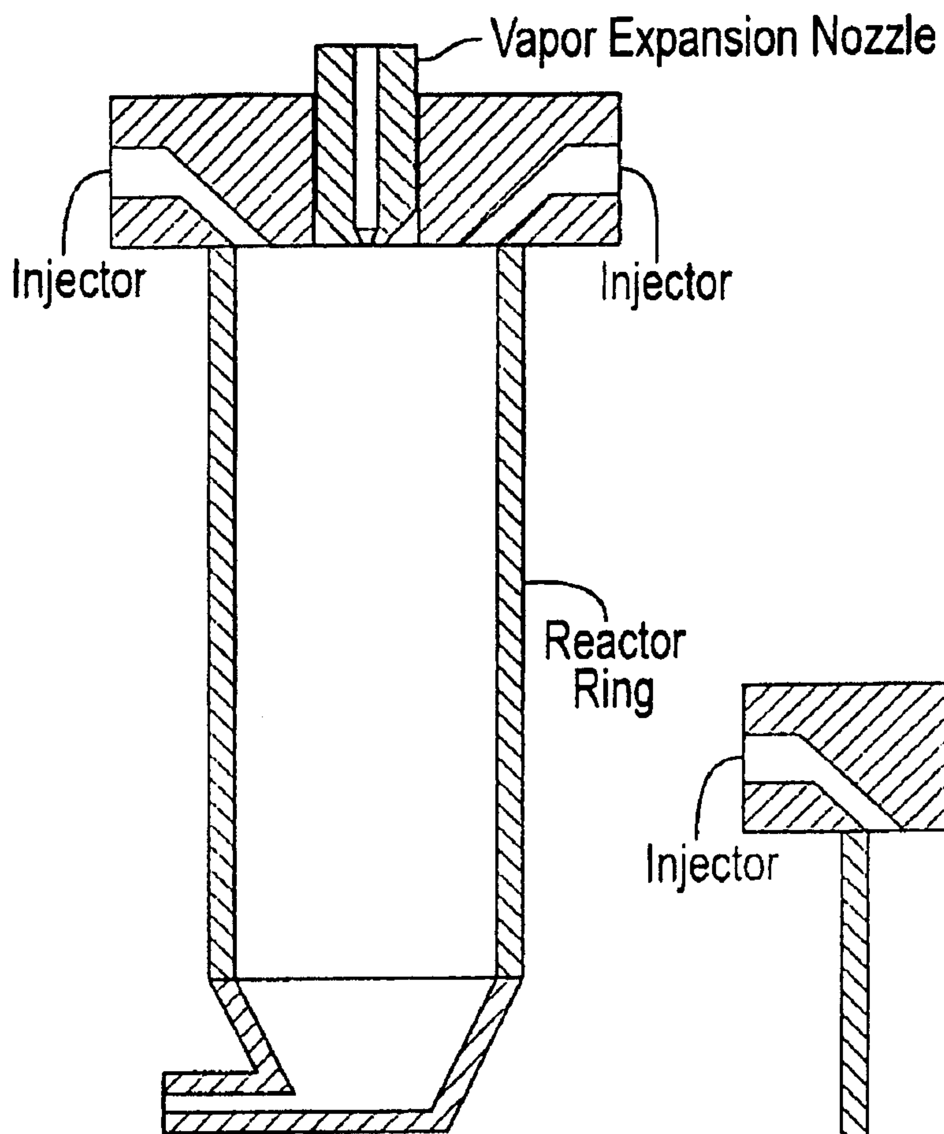
FIG. 4 (PRIOR ART)
