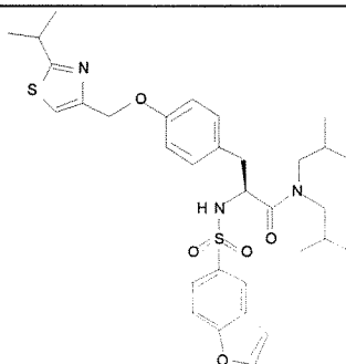
Cmpd. 155
