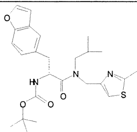
Cmpd. 159
