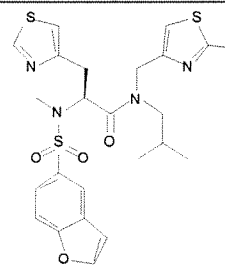
Cmpd. 80
