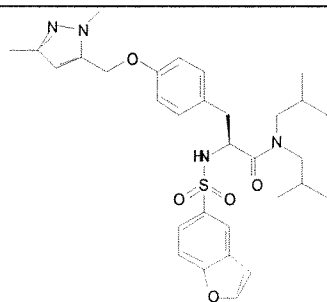
Cmpd. 159
