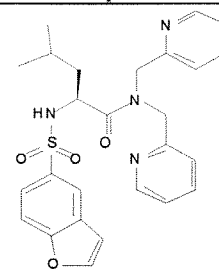
Cmpd. 26
