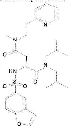
Cmpd. 41
