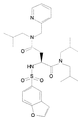
Cmpd. 40
