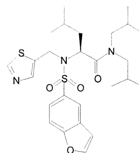
Cmpd. 138
