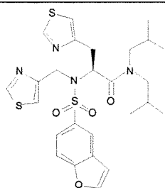
Cmpd. 147
