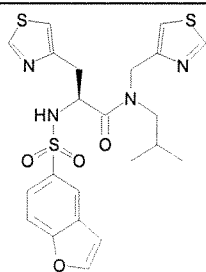
Cmpd. 123
