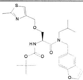
Cmpd. 19
