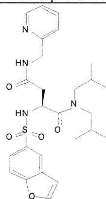
Cmpd. 38
