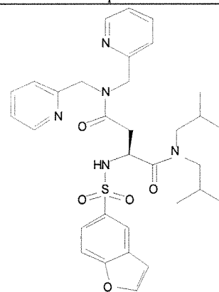
Cmpd. 42
