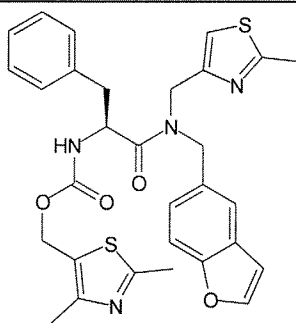
Cmpd. 131
