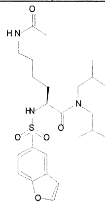
Cmpd. 81
