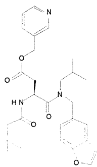
Cmpd. 67
