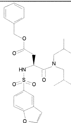
Cmpd. 36
