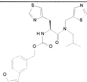
Cmpd. 173
