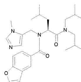
Cmpd. 130
