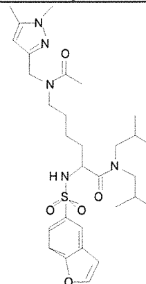
Cmpd. 82
