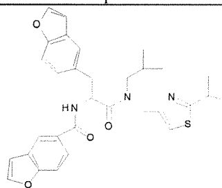
Cmpd. 169
