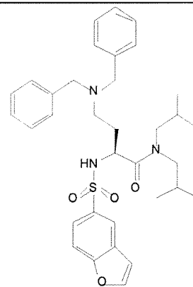
Cmpd. 78
