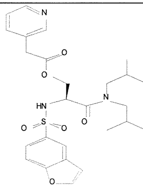
Cmpd. 32
