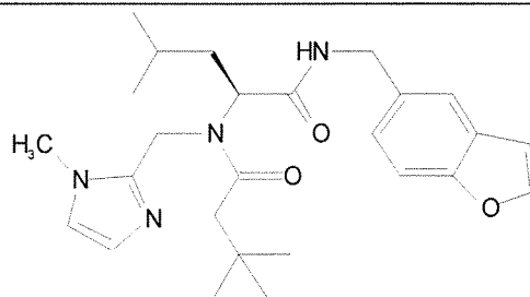
Cmpd. 20
