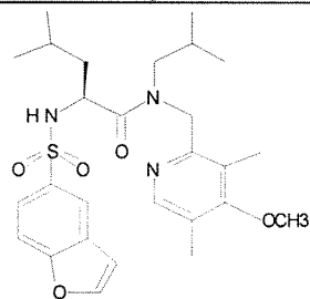
Cmpd. 27
