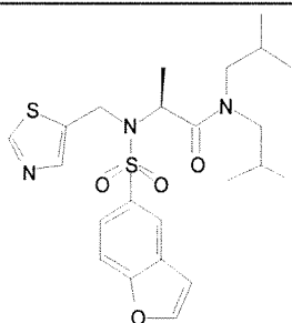
Cmpd. 151
