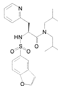
Cmpd. 72
