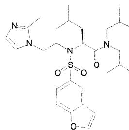
Cmpd. 156
