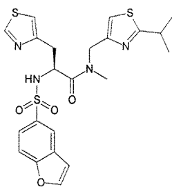
Cmpd. 125
