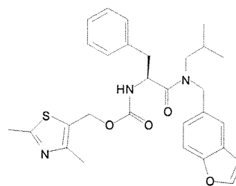
Cmpd. 132
