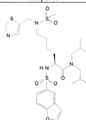
Cmpd. 136
