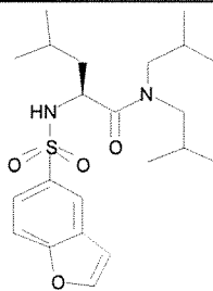
Cmpd. 21
