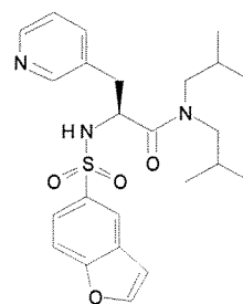
Cmpd. 48
