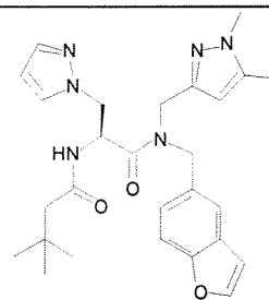
Cmpd. 76
