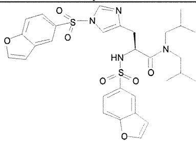
Cmpd. 49
