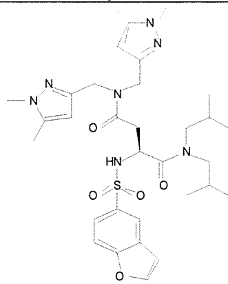
Cmpd. 45
