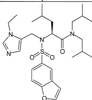
Cmpd. 141
