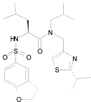
Cmpd. 31
