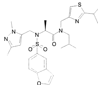
Cmpd. 160
