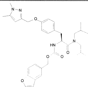
Cmpd. 175
