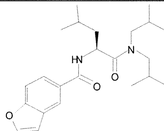
Cmpd. 22
