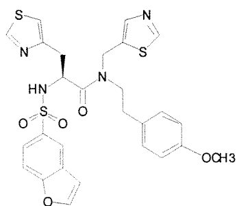
Cmpd. 176
