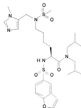
Cmpd. 140
