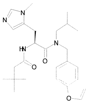
Cmpd. 69
