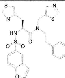
Cmpd. 166
