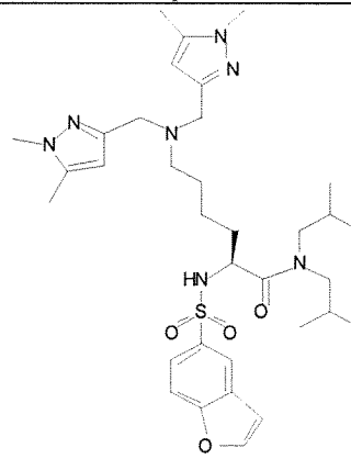
Cmpd. 34
