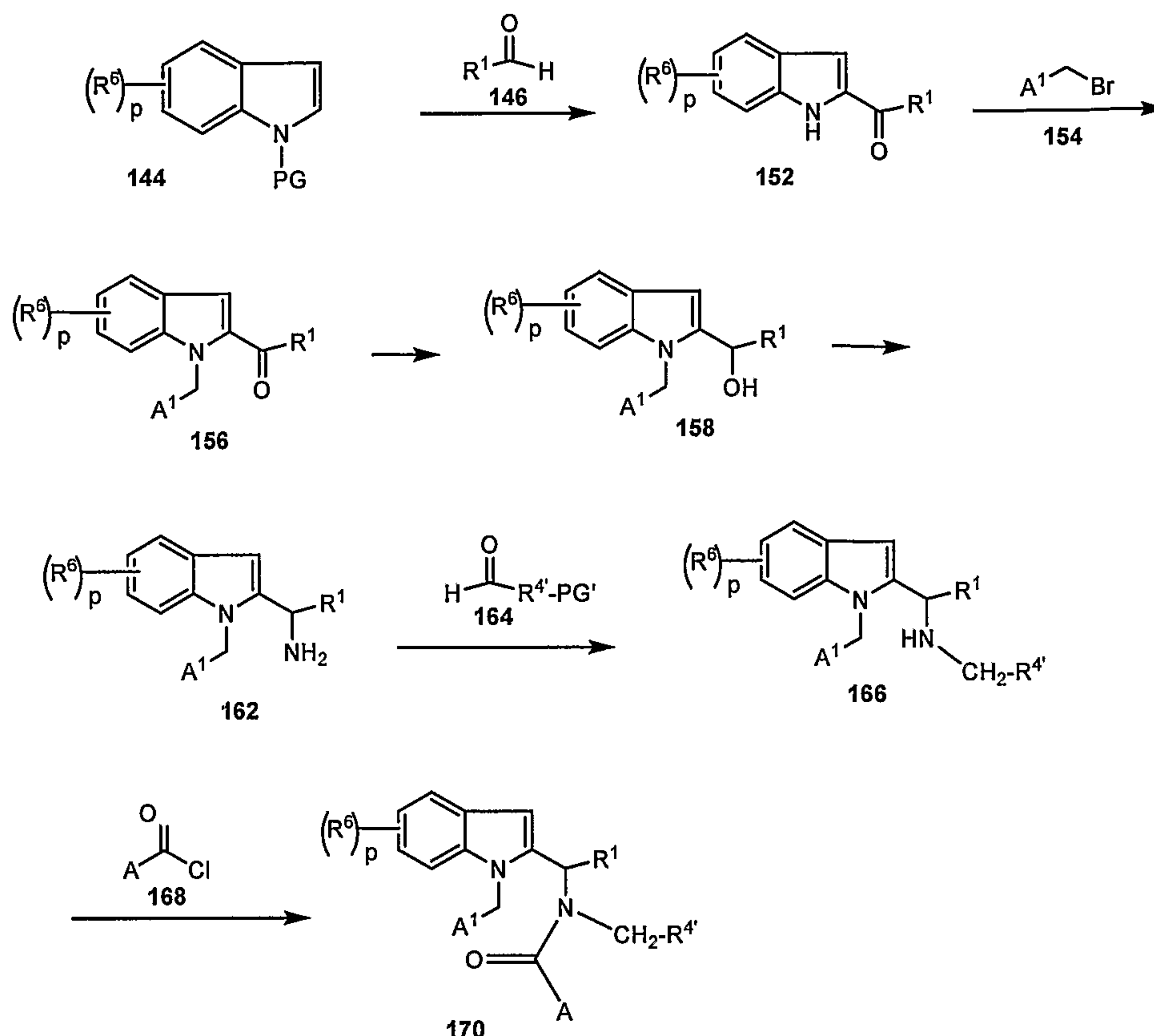
Scheme 2
