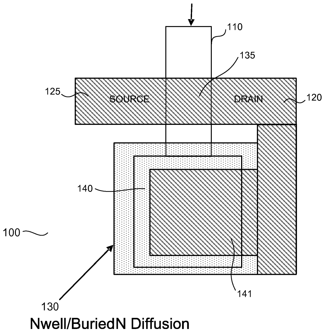
FIG. 1 Floating Gate
