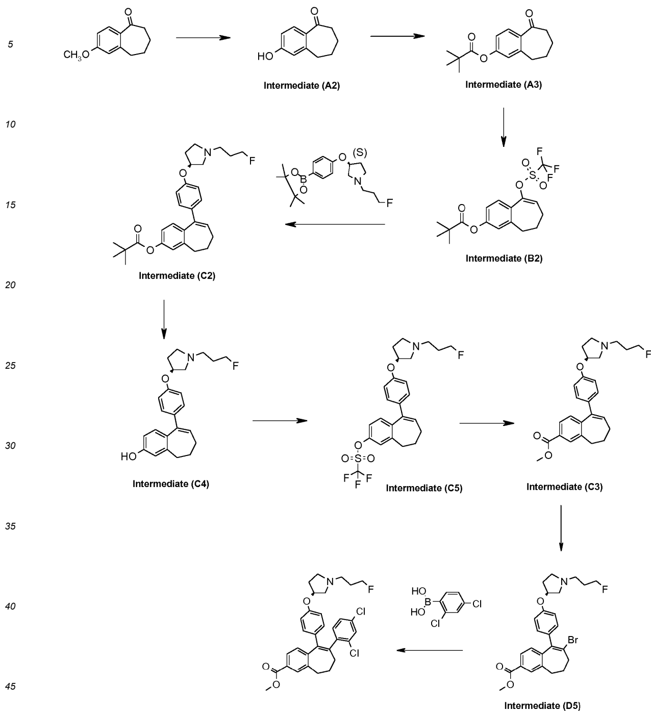
Scheme 4: Route B
