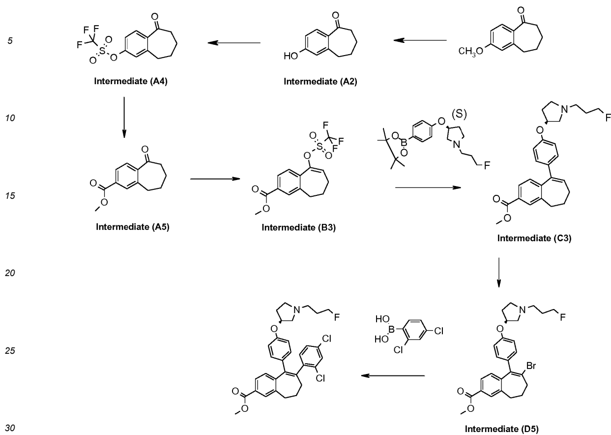
Scheme 3: Route A
