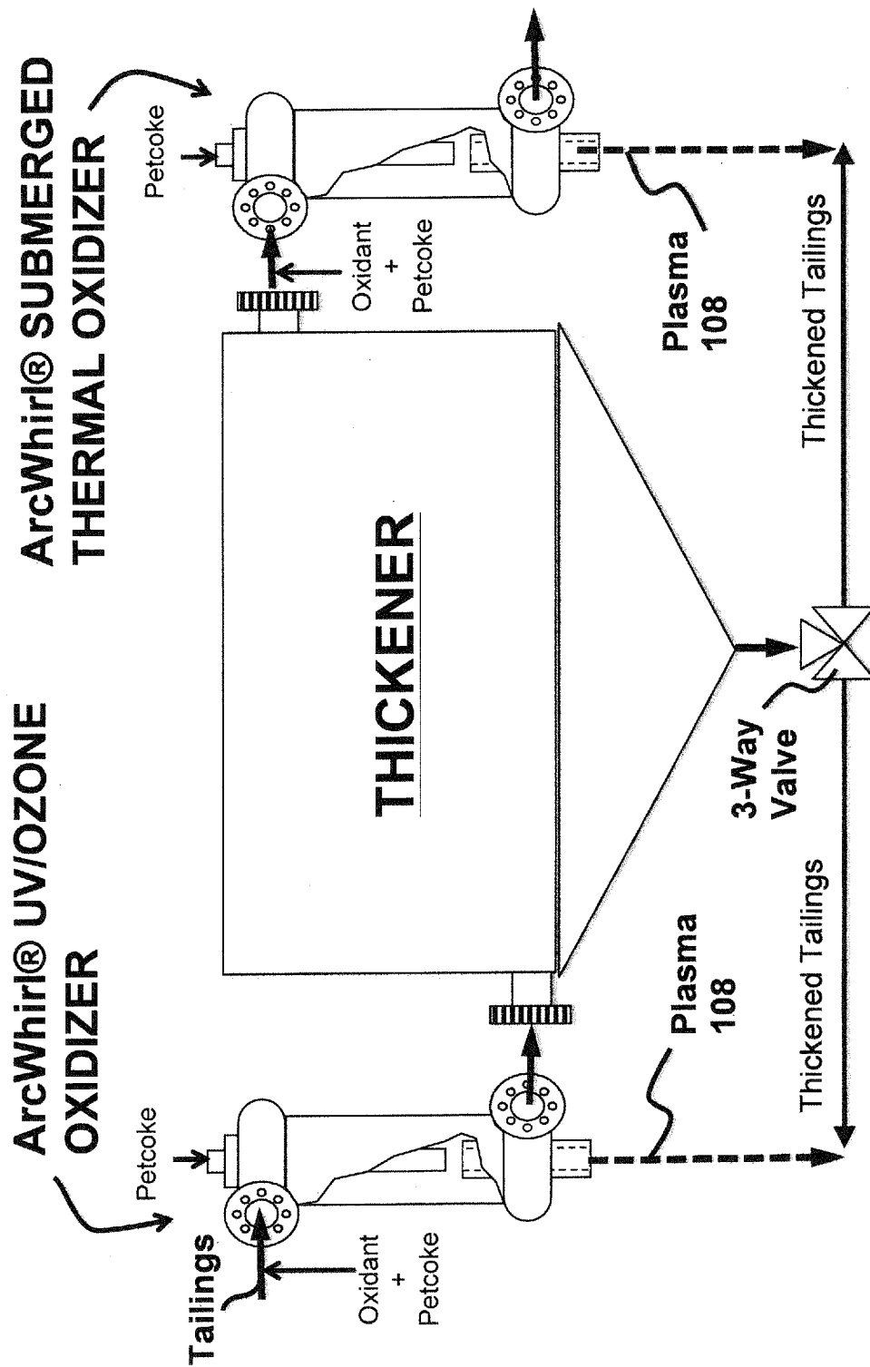
FIGURE 57 – Dual ArcWhirls® Thickener
