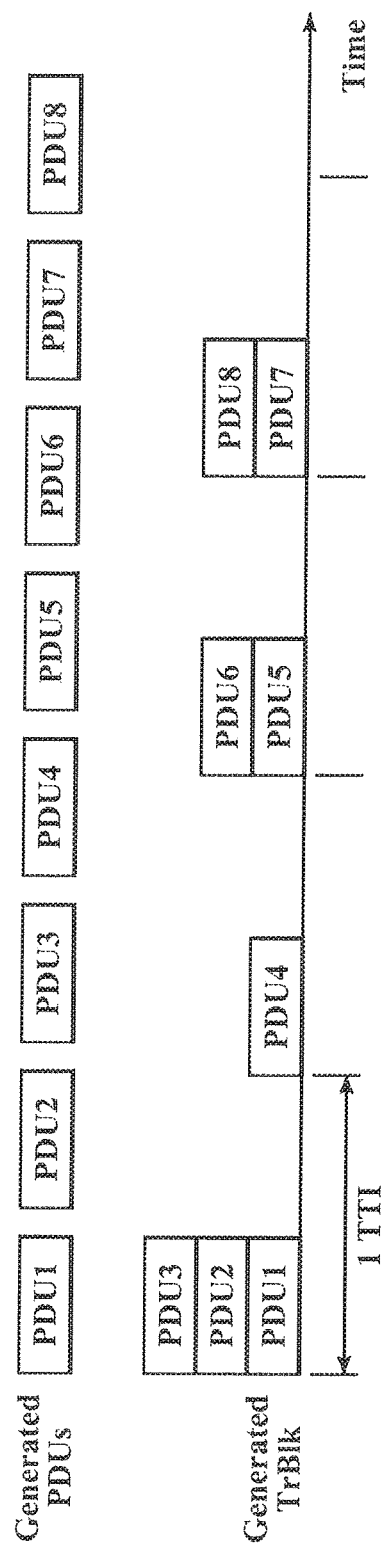
FIG. 7 - Transport Channel Block generation
