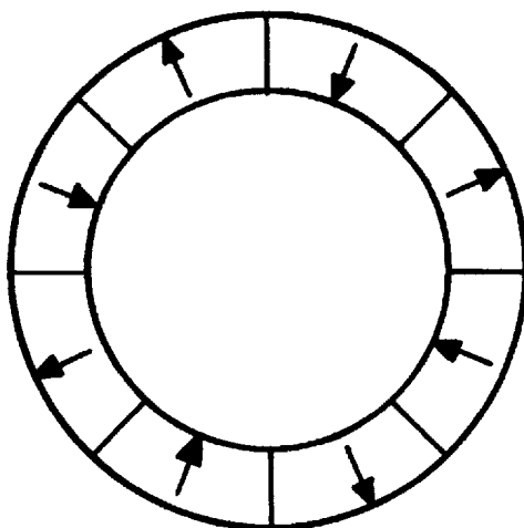
FIGURE 1 IDEALIZED EIGHT POLE RADIAL MAGNETIZATION
