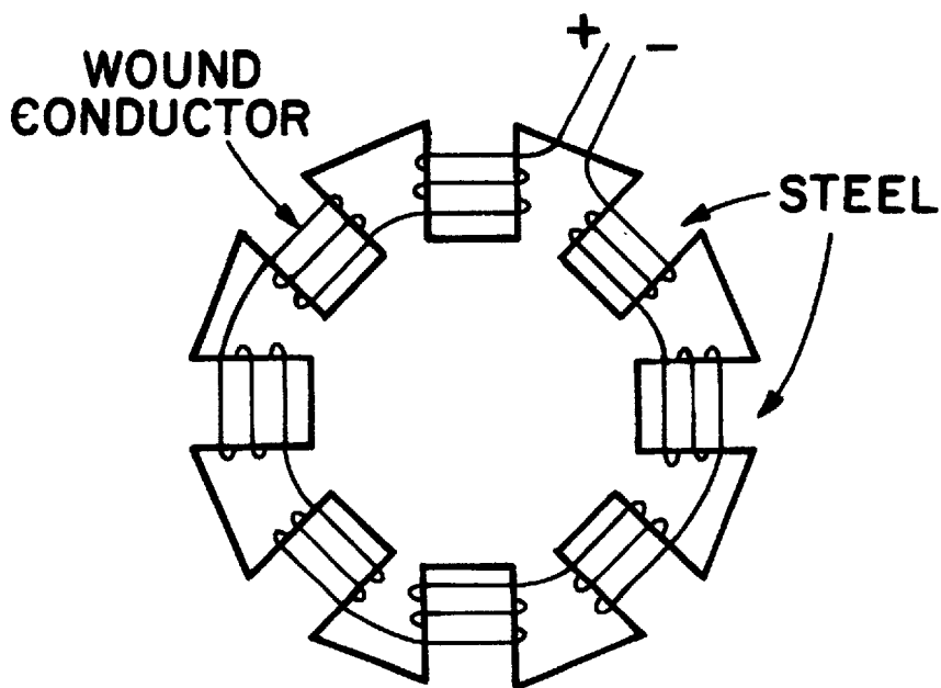
FIGURE 2 STEEL CORED MULTIPOLE FIXTURE
