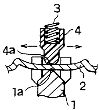
FIG. 9 PRIOR ART
