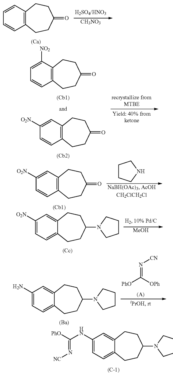
REACTION SCHEME 2
