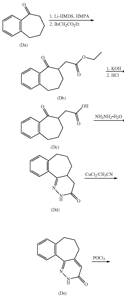
REACTION SCHEME 3
