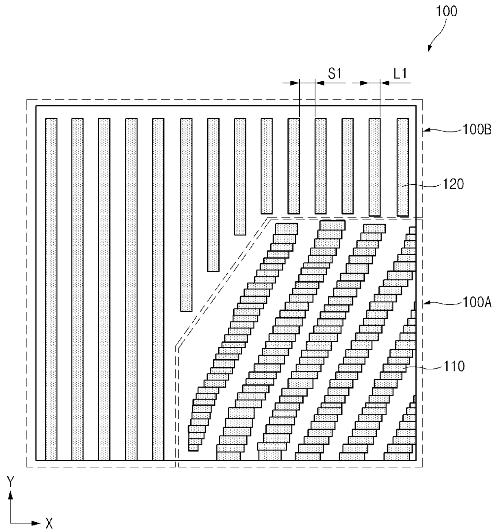
Fig.1 <Prior Art>
