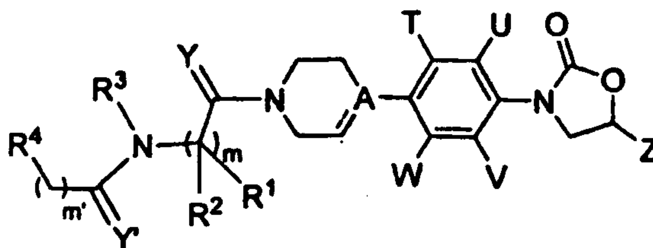
Formula I
