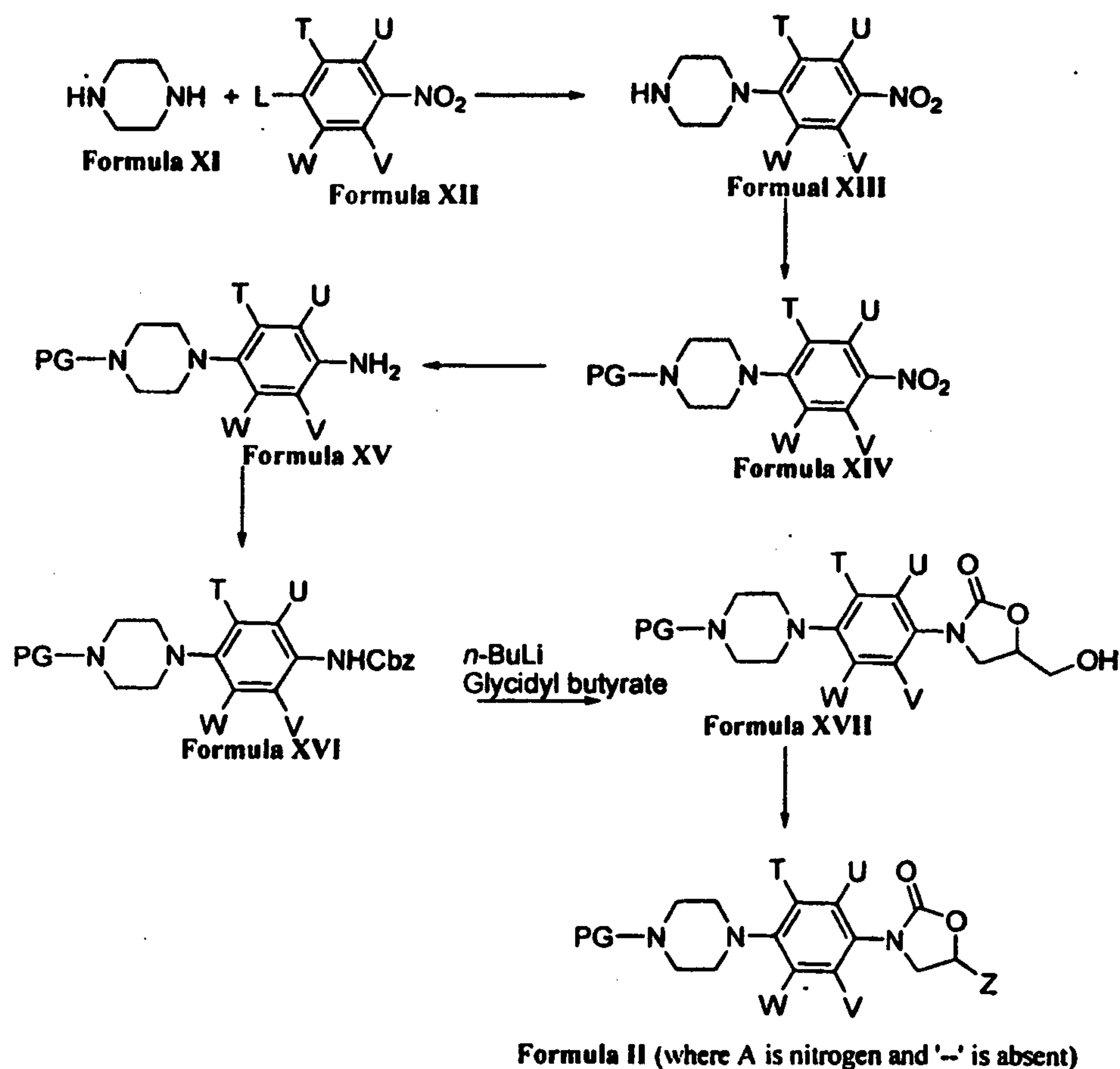
Scheme 3
