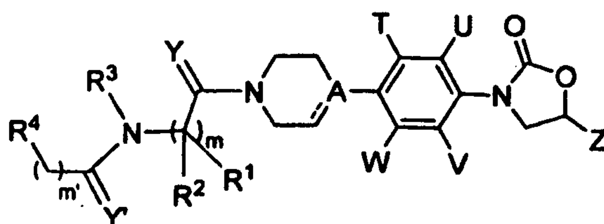
Formula I
