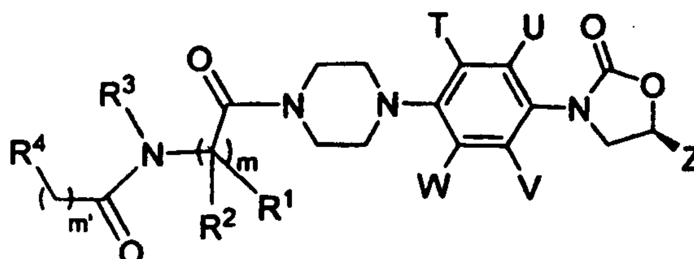
Formula Ib
