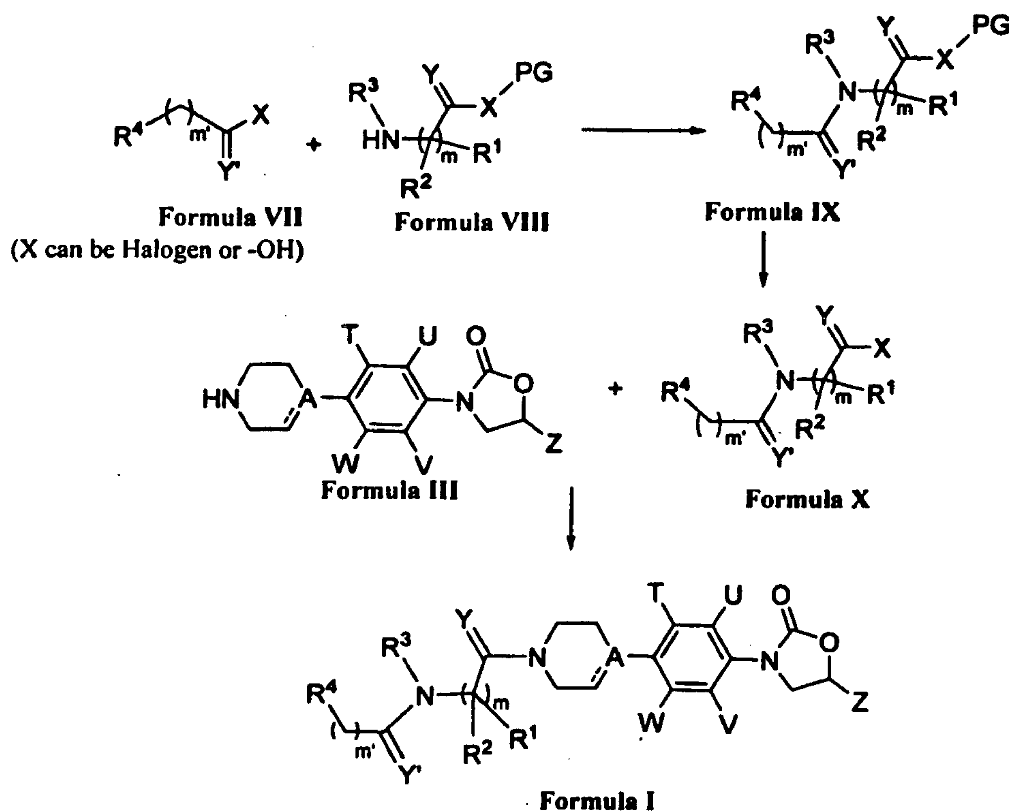
Scheme 2
