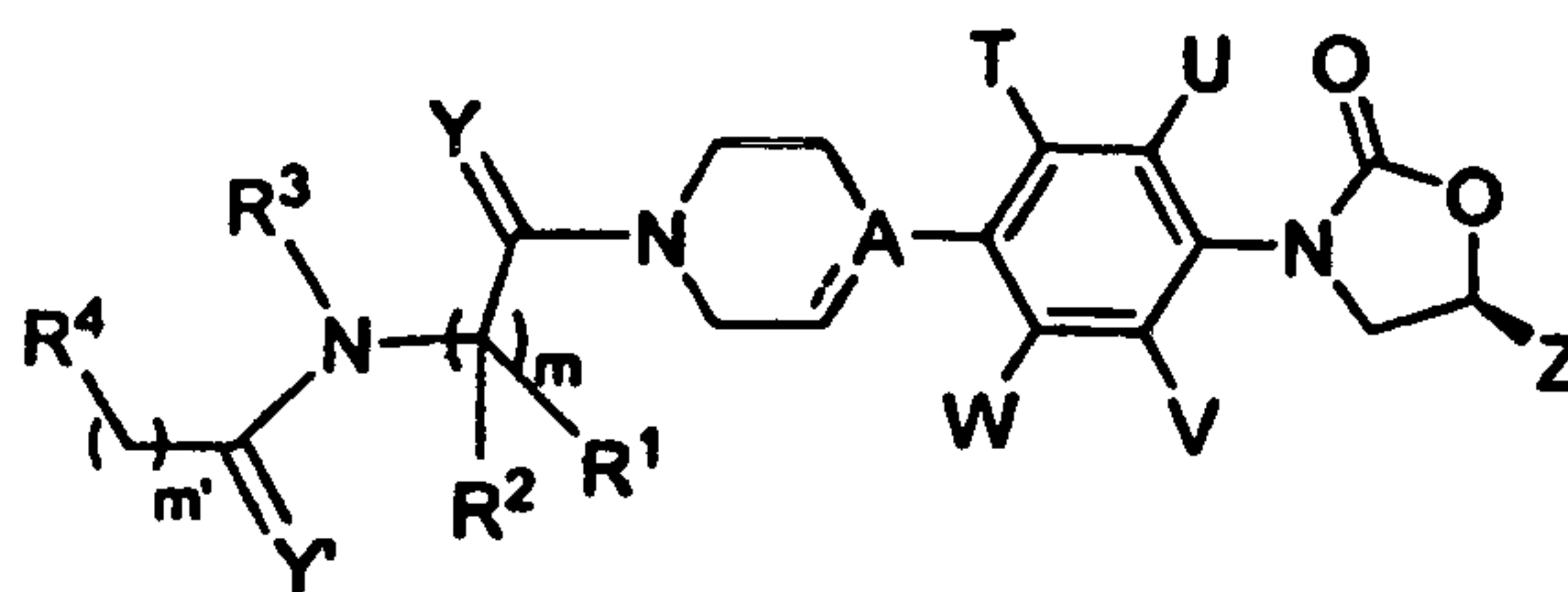
Formula Ia
