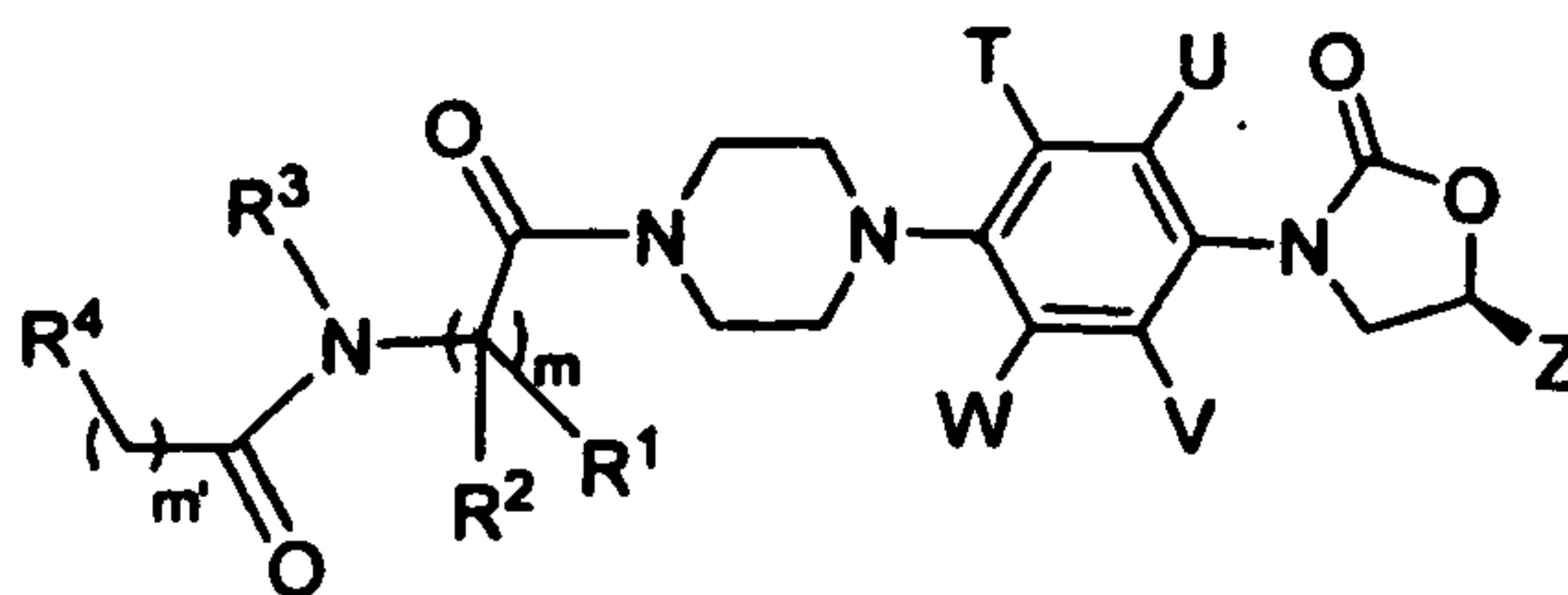
Formula Ib
