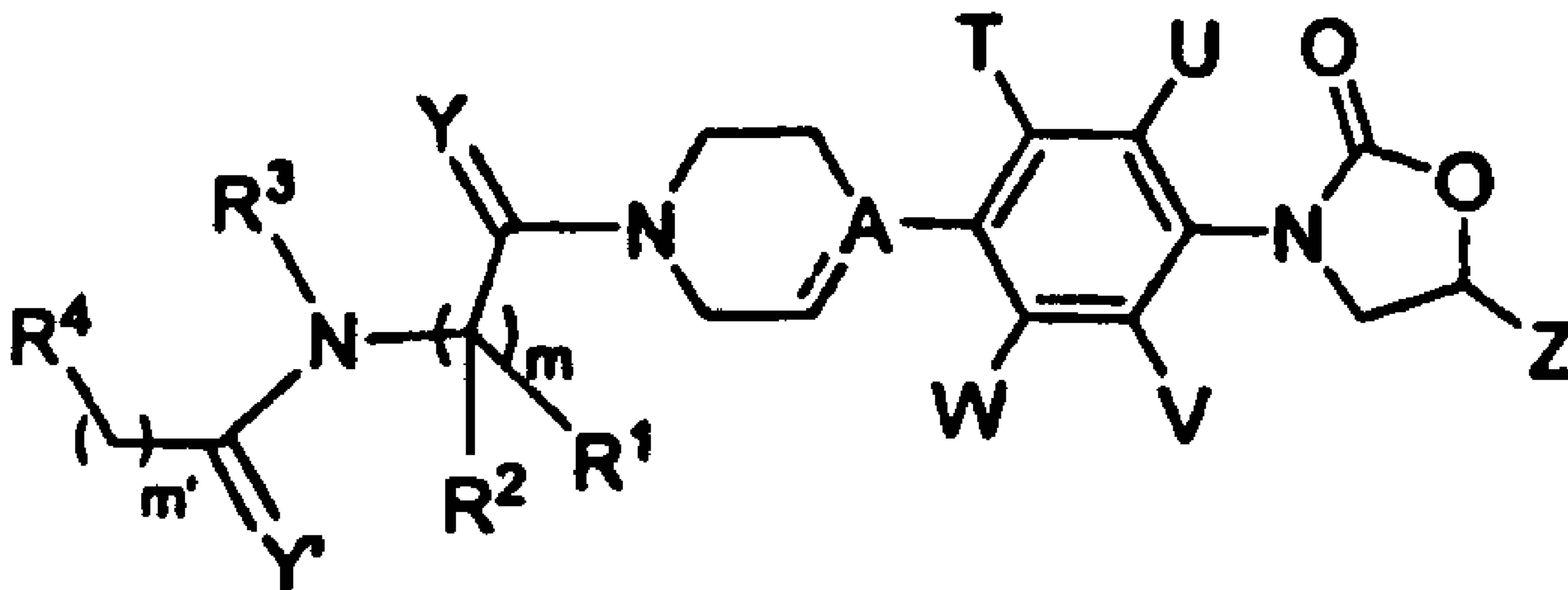
Formula I
