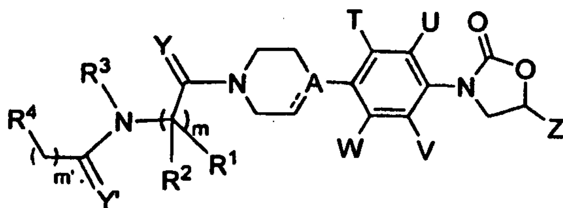
Formula I
