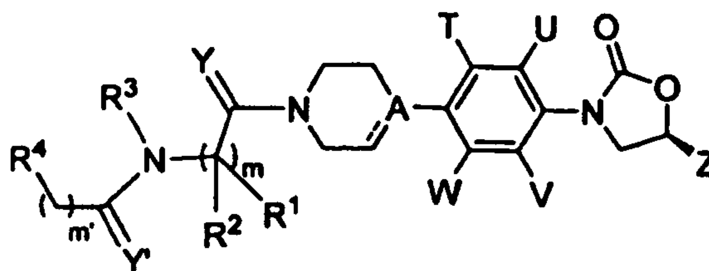
Formula Ia
