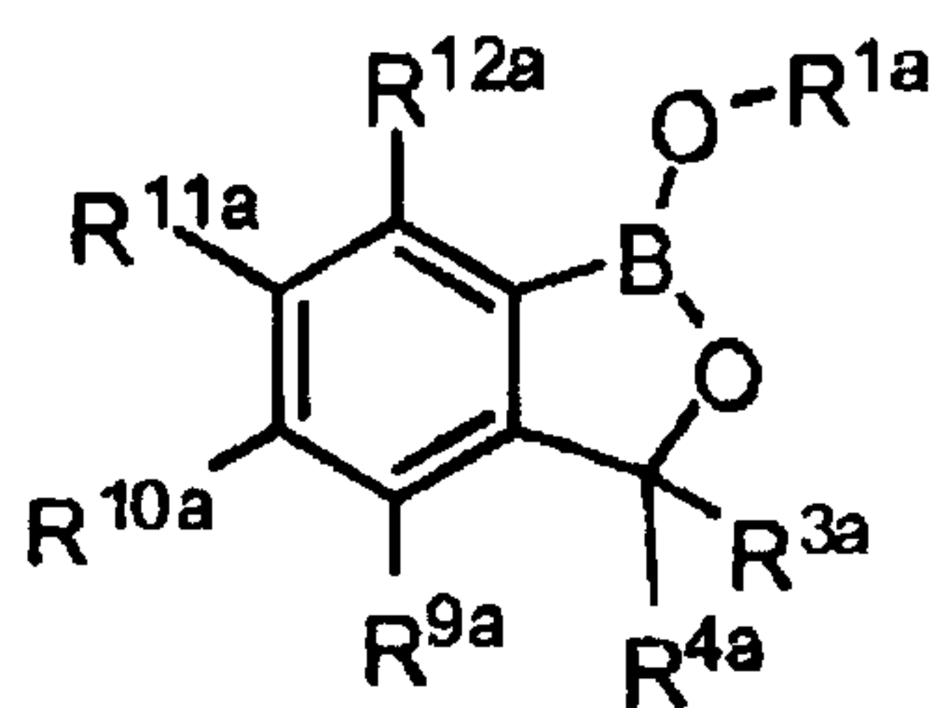
Formula Ia.
