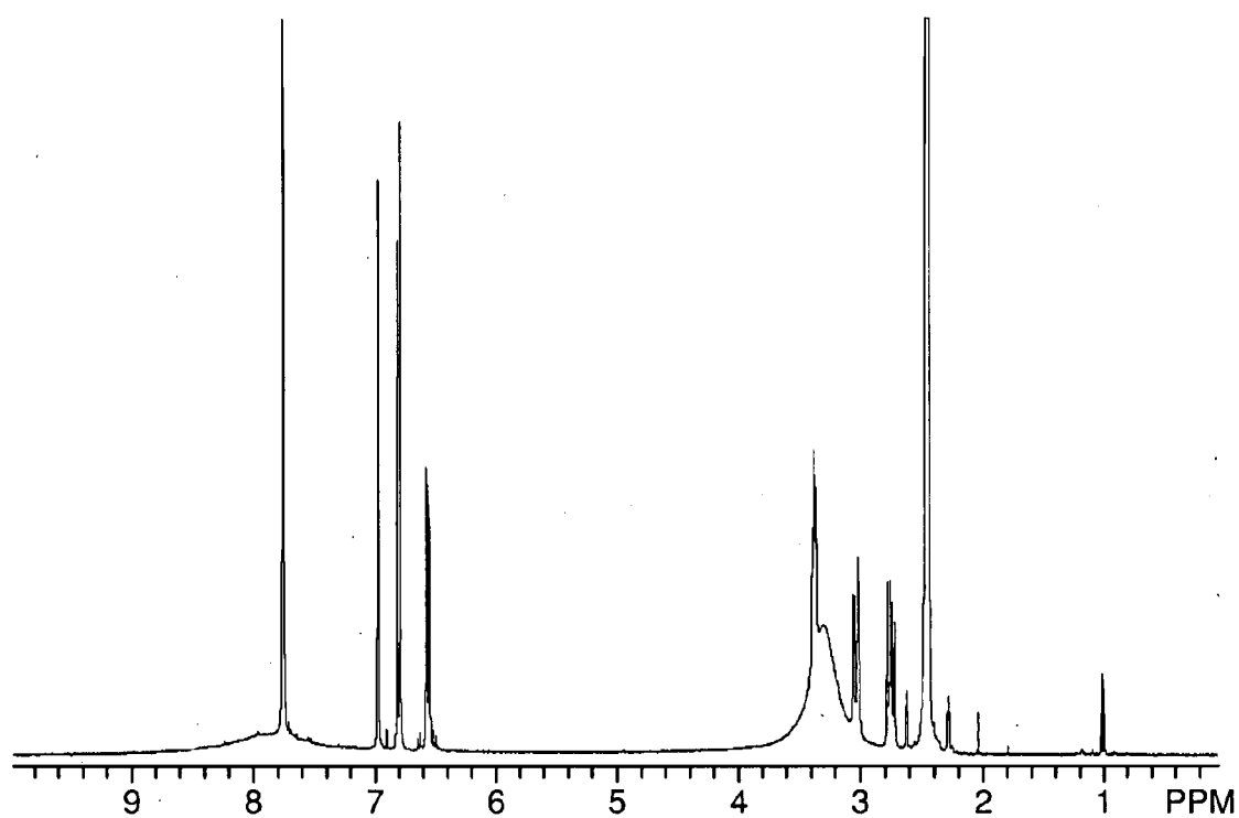
Proton NMR of Triiodothyronine (T3)
