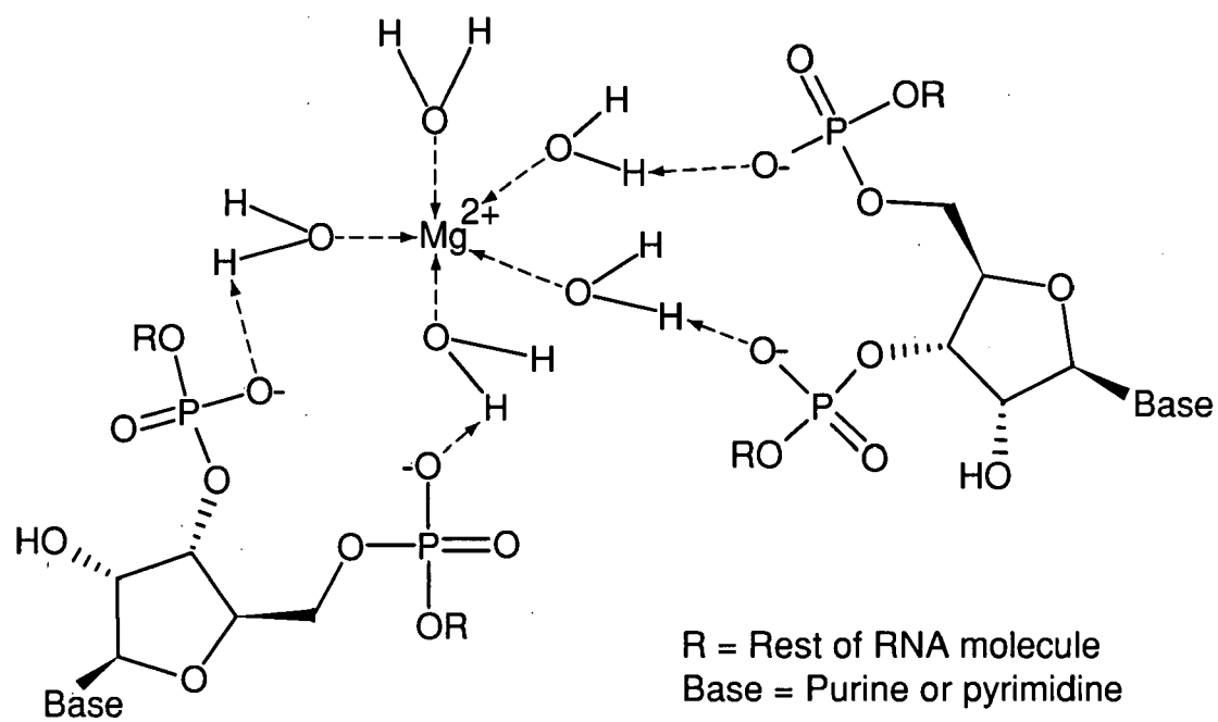
Outer sphere RNA:Magnesium Coordination Complex
