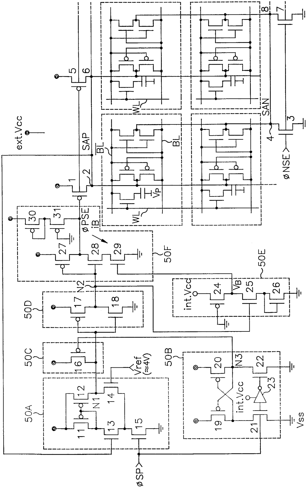
FIG. 2 (PRIOR ART)
