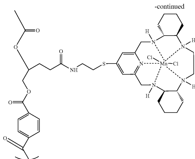
Poly(ethylene terephthalate) with surface bound PACPeD catalyst
