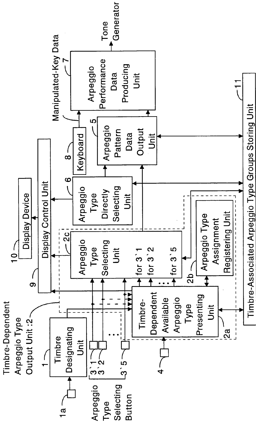
Fig. 1 Functional Configuration
