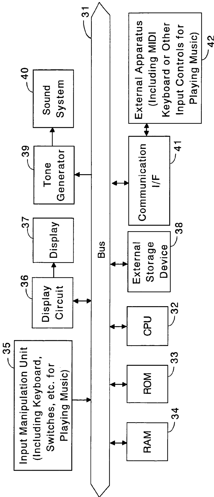
Fig. 4 Hardware Configuration
