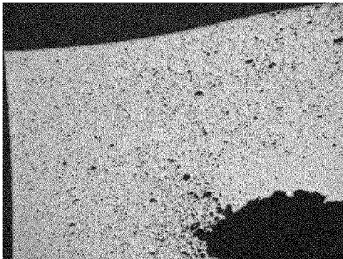
Figure 4. Void inside sintered specimen from trial #1.
