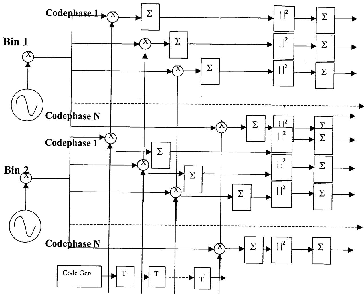
FIGURE 8-2 BIN SEARCH ENGINE ARCHITECTURE
