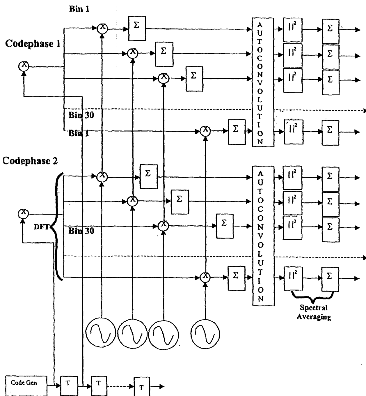
FIGURE 9 - 2 CODEPHASE MODIFIED SEARCH ENGINE
