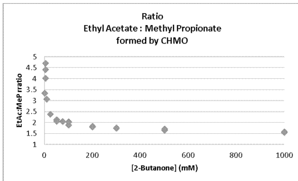
Figure 1. Conversion of different concentrations of 2-butanone by 5 \mu M CHMO. Each reaction in 1 mL 50 mM Tris-HCl, pH 7.5, containing 100 \mu M NADPH and 10 mM \text{Na}_2\text{HPO}_3 at room temperature for 24 hours.
