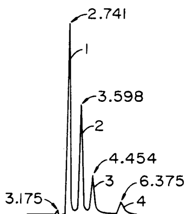
FIG. 9b 48 HRS at pH=10 N=19,000
