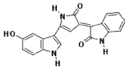
Violacein (2)
