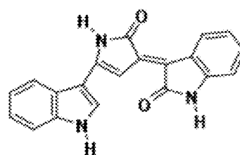
Deoxyviolacein (3)
