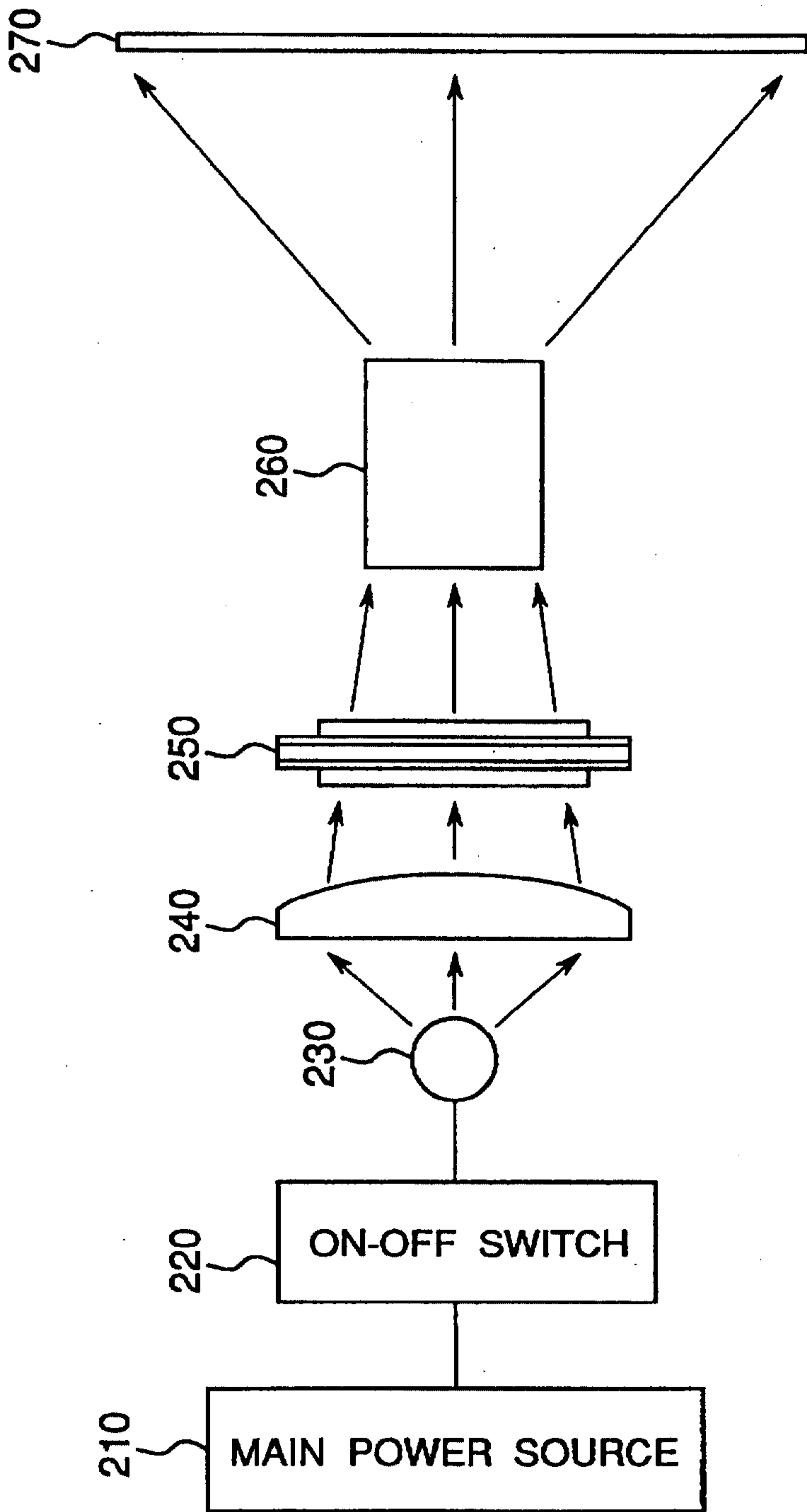
Fig. 14 PRIOR ART
