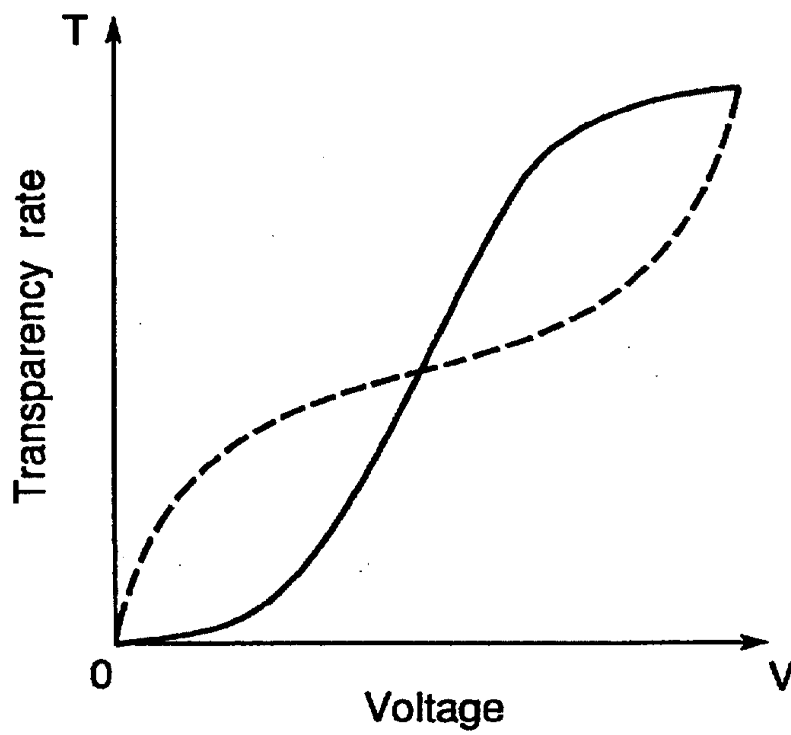
Fig.15 PRIOR ART
