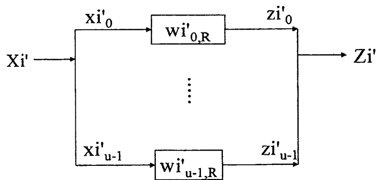
FIG. 26 Nonlinear Transform
