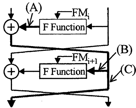
Propagation of Mask in Feistel Encryption
