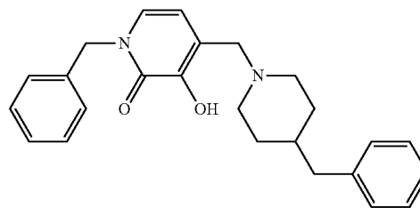
1-Benzyl-3-hydroxy-4-(4-benzylpiperidin-1-ylmethyl)pyridin-2(1H)-one
