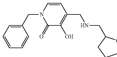
1-Benzyl-3-hydroxy-4-[(tetrahydrofuran-2-ylmethyl)amino]methylpyridin-2(1H)-one
