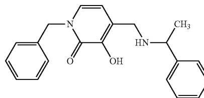
1-Benzyl-3-hydroxy-4-[(1-phenylethylamino)methyl]pyridin-2(1H)-one
