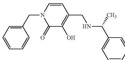
(R)-1-Benzyl-3-hydroxy-4-[(1-phenylethylamino)methyl]pyridin-2(1H)-one
