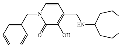
1-Benzyl-3-hydroxy-4-(cycloheptylaminomethyl)pyridin-2(1H)-one
