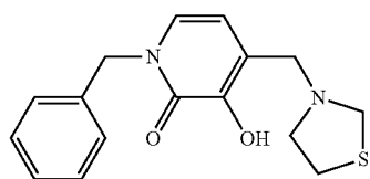
1-Benzyl-3-hydroxy-4-(thiazolidin-3-ylmethyl)pyridin-2(1H)-one
