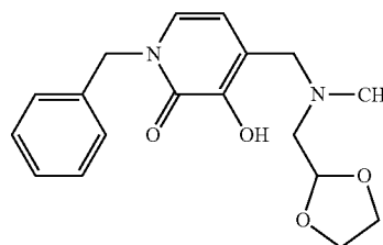
1-Benzyl-3-hydroxy-4-[(1,3-dioxolan-2-ylmethyl)methylamino]methyl]pyridin-2(1H)-one
