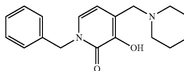
1-Benzyl-3-hydroxy-4-(piperidin-1-ylmethyl)pyridin-2(1H)-one
