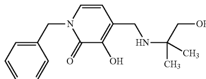
1-Benzyl-3-hydroxy-4-[(1-hydroxy-2-methylpropan-2-ylamino)methyl]pyridin-2(1H)-one
