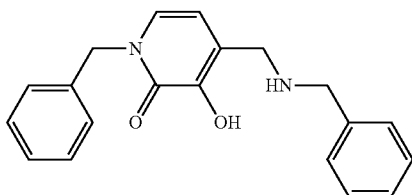
1-Benzyl-3-hydroxy-4-(benzylaminomethyl)pyridin-2(1H)-one
