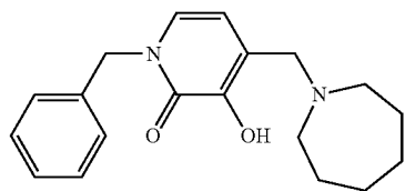
1-Benzyl-3-hydroxy-4-azepan-1-ylmethylpyridin-2(1H)-one
