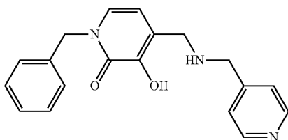
1-Benzyl-3-hydroxy-4-[(pyridin-4-ylmethylamino)methyl]pyridin-2(1H)-one
