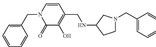
1-Benzyl-3-hydroxy-4-[(1-benzylpyrrolidin-3-ylamino)methyl]pyridin-2(1H)-one
