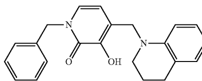
1-Benzyl-3-hydroxy-4-[(3,4-dihydroquinolin-1(2H)-yl)methyl]pyridin-2(1H)-one
