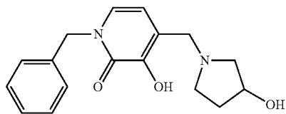
1-Benzyl-3-hydroxy-4-[(3-hydroxypyrrolidin-1-yl)methyl]pyridin-2(1H)-one
