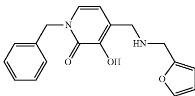
1-Benzyl-3-hydroxy-4-[(furan-2-ylmethylamino)methyl]pyridin-2(1H)-one
