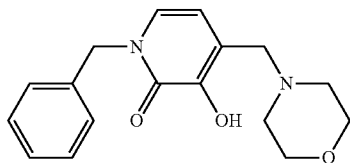
1-Benzyl-3-hydroxy-4-(morpholin-4-ylmethyl)pyridin-2(1H)-one
