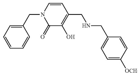
1-Benzyl-3-hydroxy-4-[(4-methoxybenzylamino)methyl]pyridin-2(1H)-one
