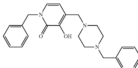
1-Benzyl-3-hydroxy-4-(4-benzylpiperazin-1-ylmethyl)pyridin-2(1H)-one
