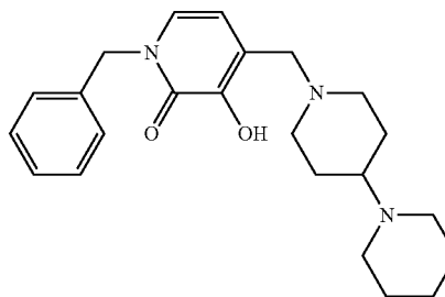
1-Benzyl-3-hydroxy-(1,4'-bipiperidinyl-1'-ylmethyl)pyridin-2(1H)-one
