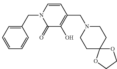
1-Benzyl-3-hydroxy-4-(1,4-dioxo-8-azaspiro[4,5]dec-8-ylmethyl)pyridin-2(1H)-one
