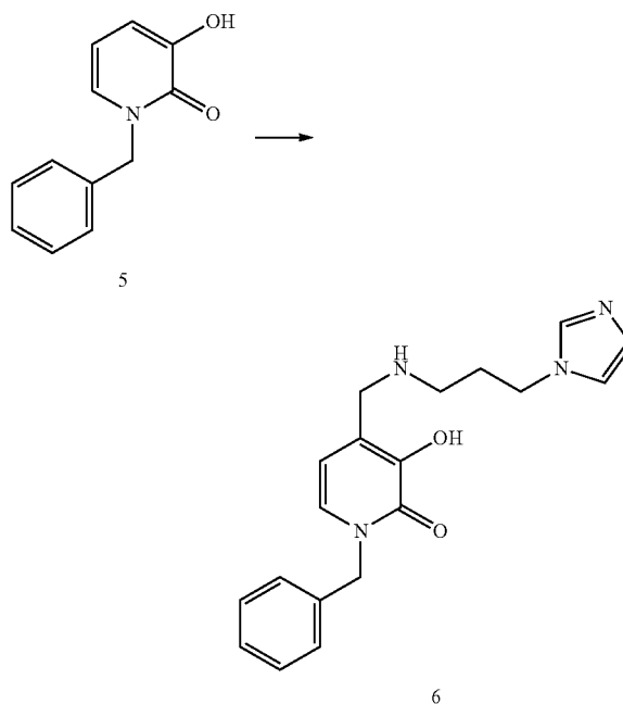
Scheme II
