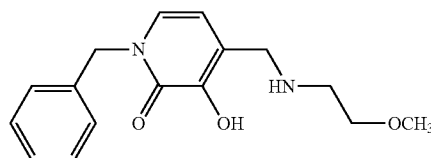
1-Benzyl-3-hydroxy-4-[(2-methoxyethylamino)methyl]pyridin-2(1H)-one
