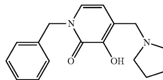
1-Benzyl-3-hydroxy-4-(pyrrolidin-1-ylmethyl)pyridin-2(1H)-one
