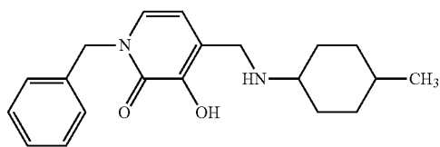
1-Benzyl-3-hydroxy-4-[(4-methylcyclohexylamino)methyl]pyridin-2(1H)-one
