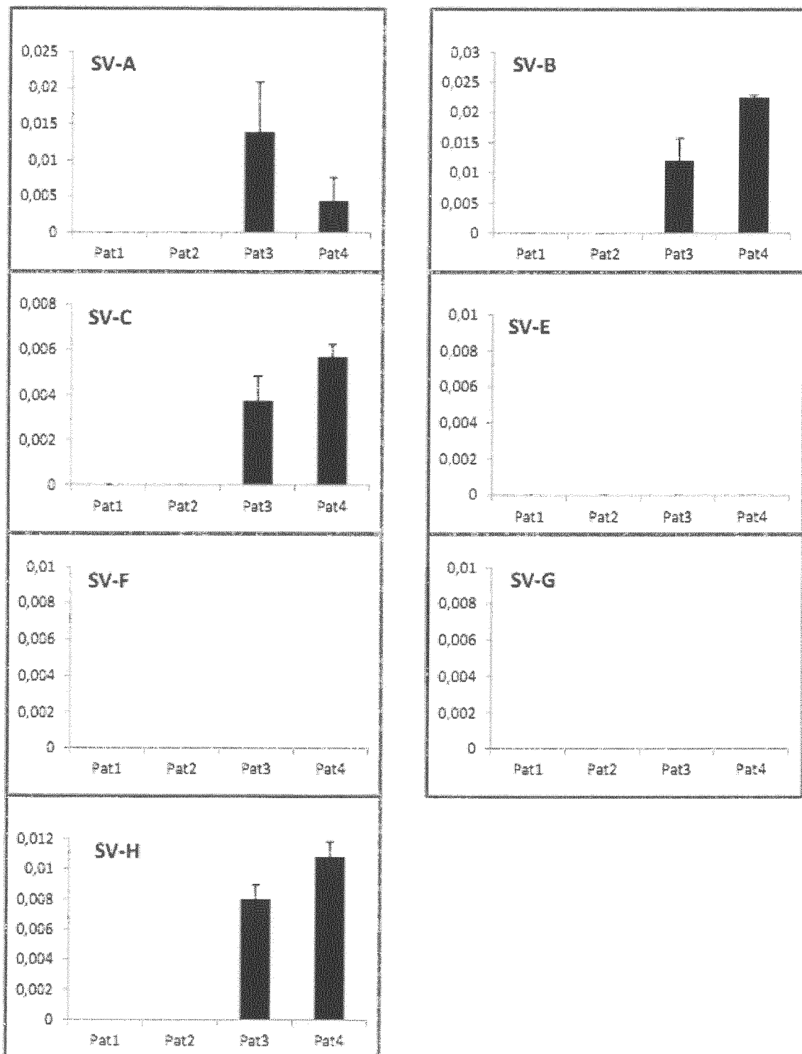
Fig. 8 AGR2 SVs mRNA levels in exosomes isolated from the urine of 4 patients with renal cell carcinoma
