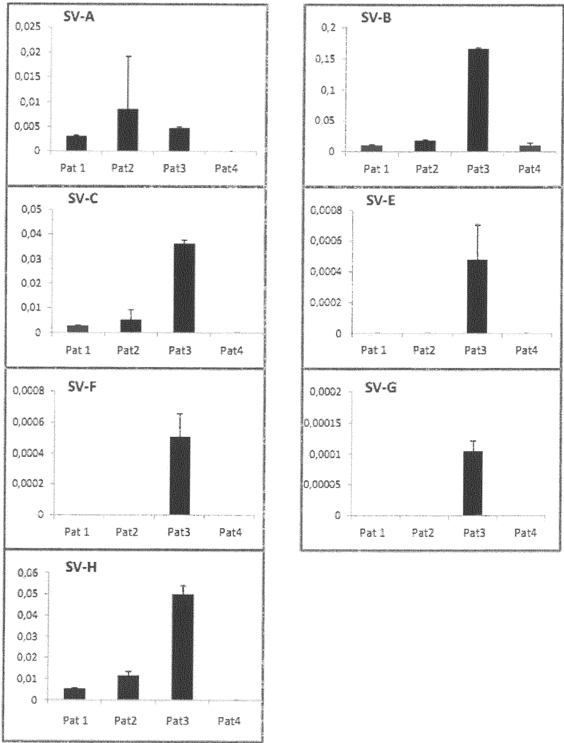
Fig. 7 AGR2 SVs mRNA levels in exosomes isolated from the urine of 4 patients with urothelial carcinoma
