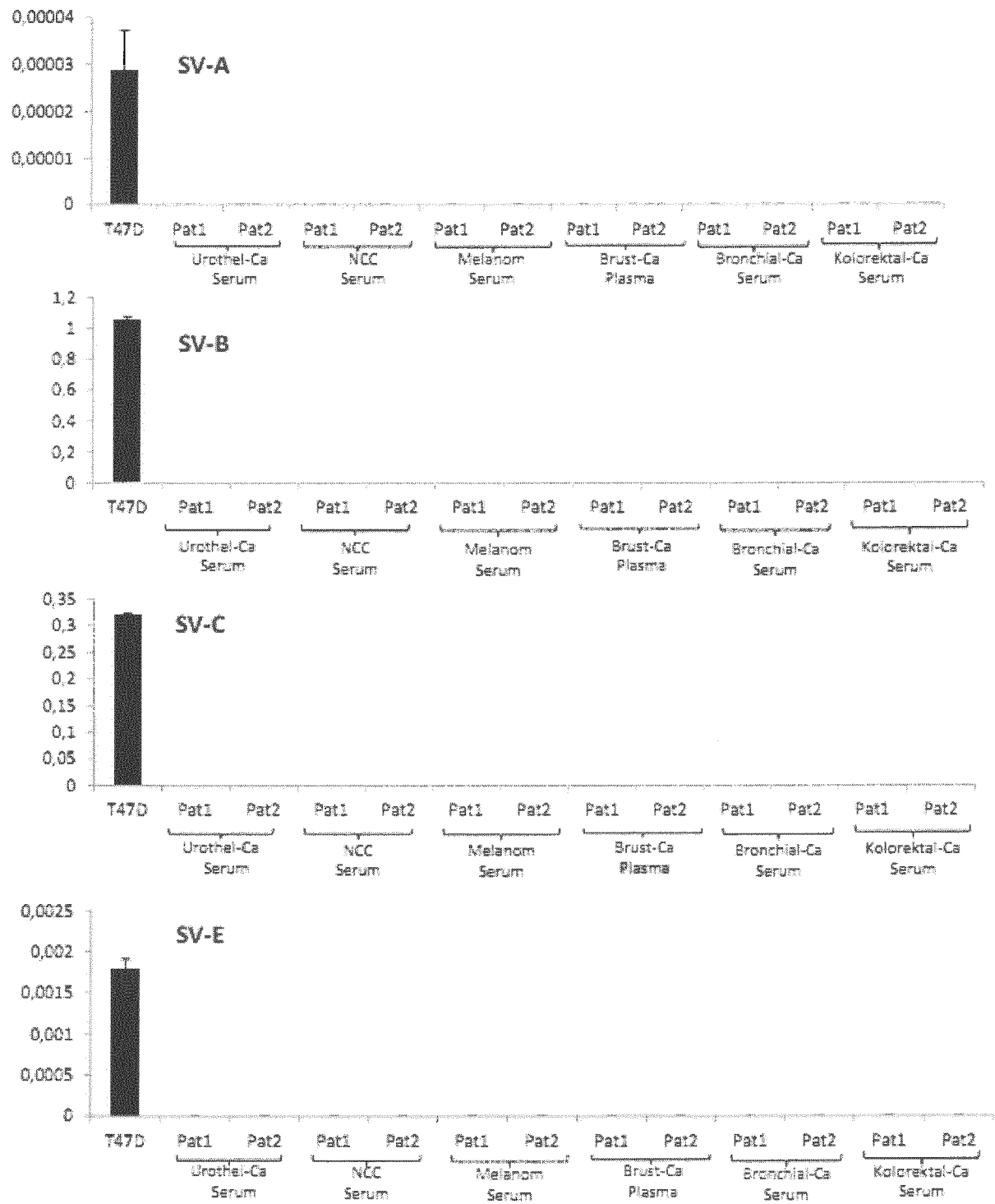
Fig. 9A AGR2 SVs mRNA levels in exosomes isolated from blood (serum or plasma) of patients with different tumor types
