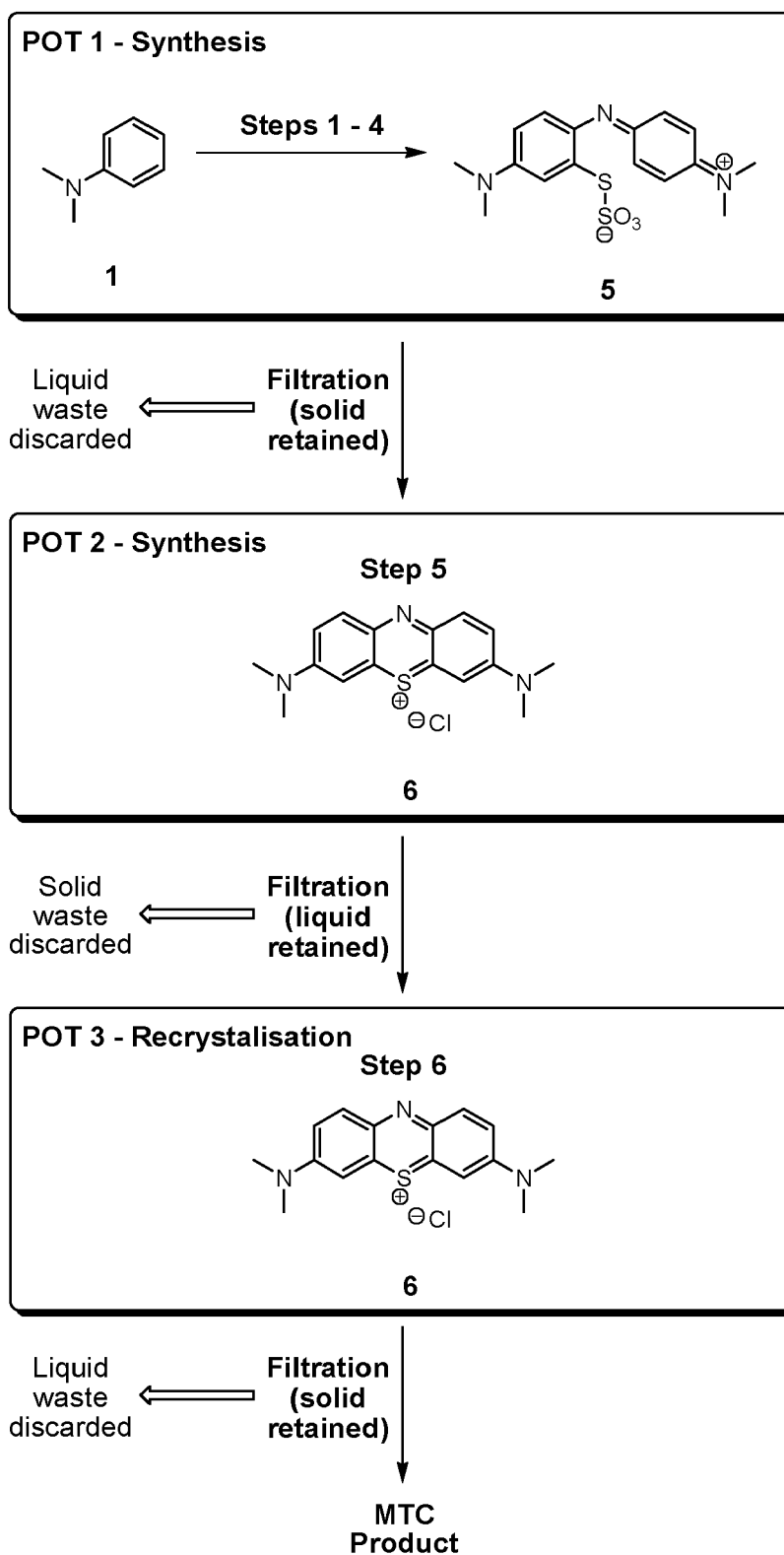
Scheme 1 – Synthesis by a 3-pot process
