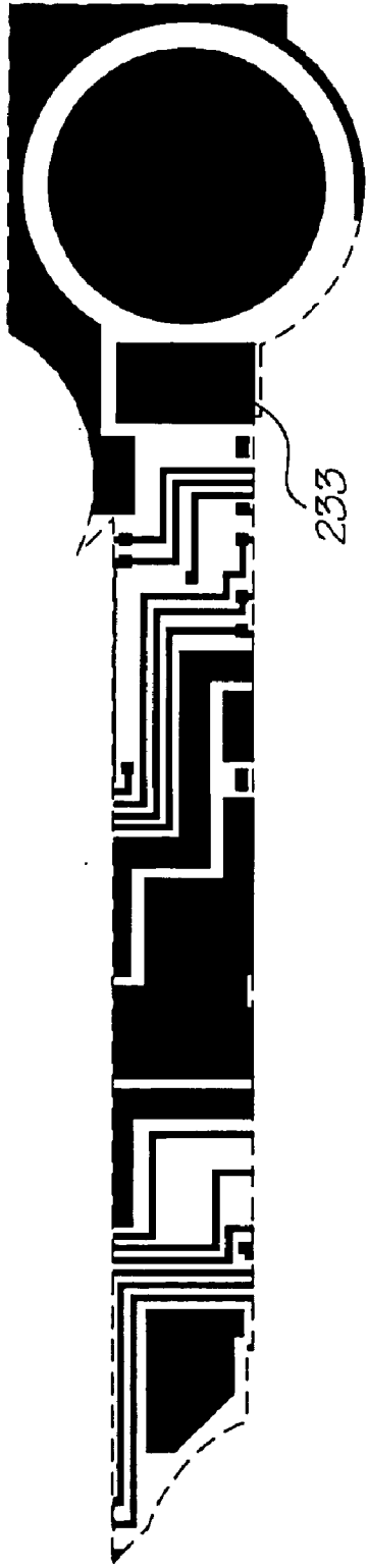
Metal 2 mask
