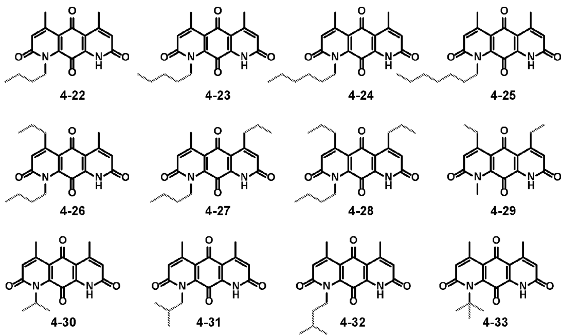
Scheme 4.3. New DNQ derivatives.
