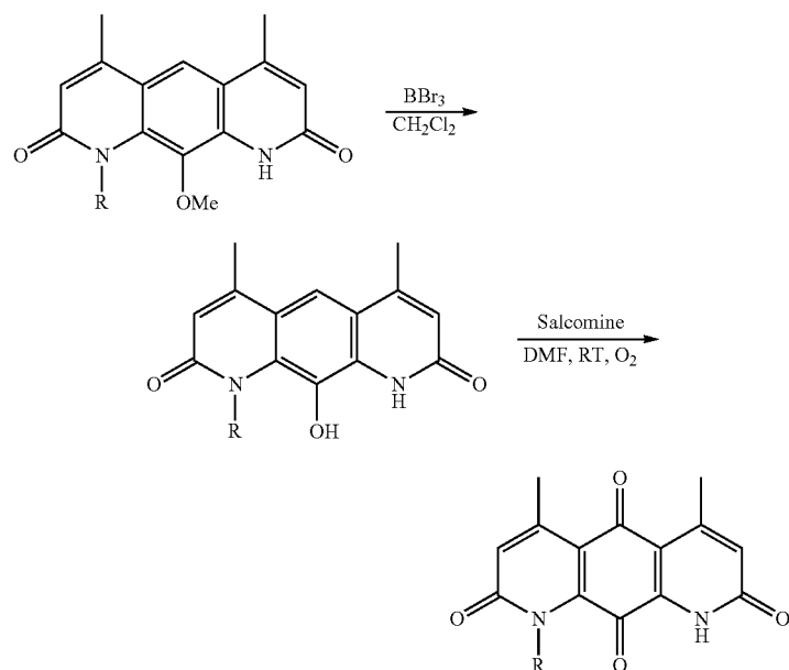
Scheme 4.5. Synthesis of DNQ derivatives bearing substituents sensitive to HBr-mediated deprotection.
