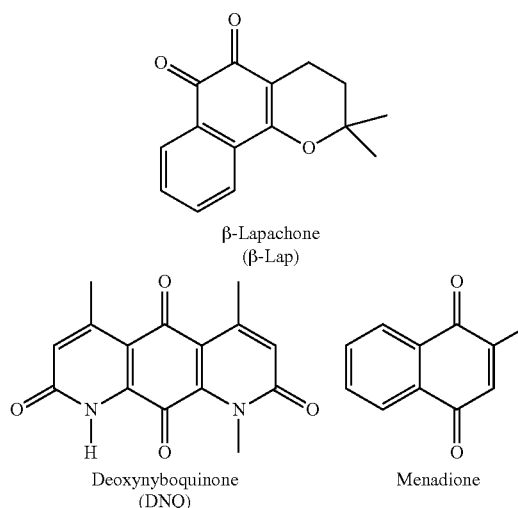
Scheme 1. Example of Quinone Compounds.
