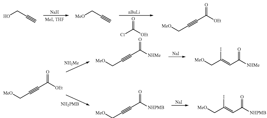
Scheme 7.2. Preparation of DNQ-P2 and DNQ-P3 Intermediates.
