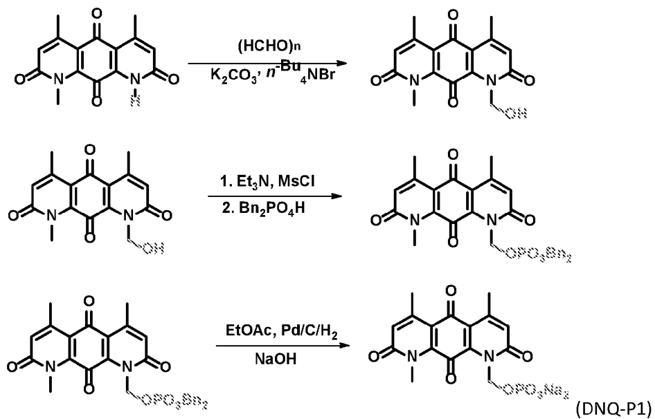
Scheme 7.1. Preparation of DNQ-P1.
