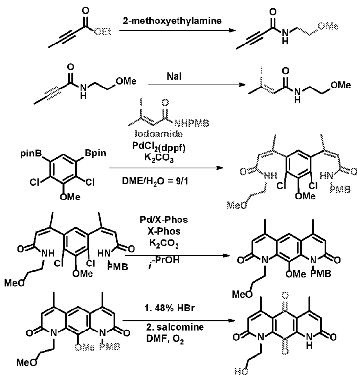
Scheme 7.4. Preparation of DNQ-P4.
