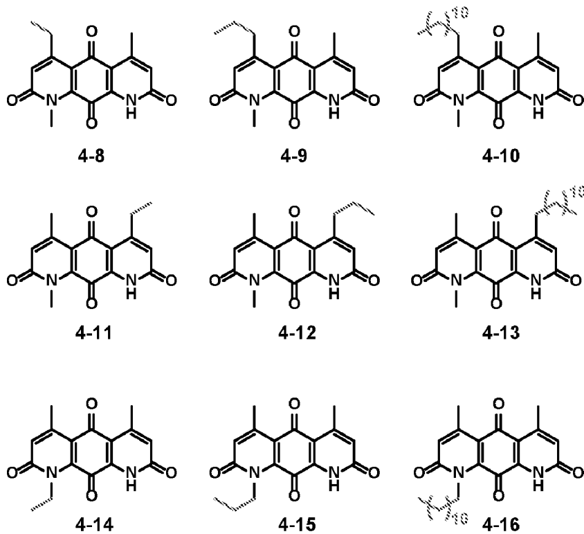
Scheme 4.1. Nine DNQ derivatives.
