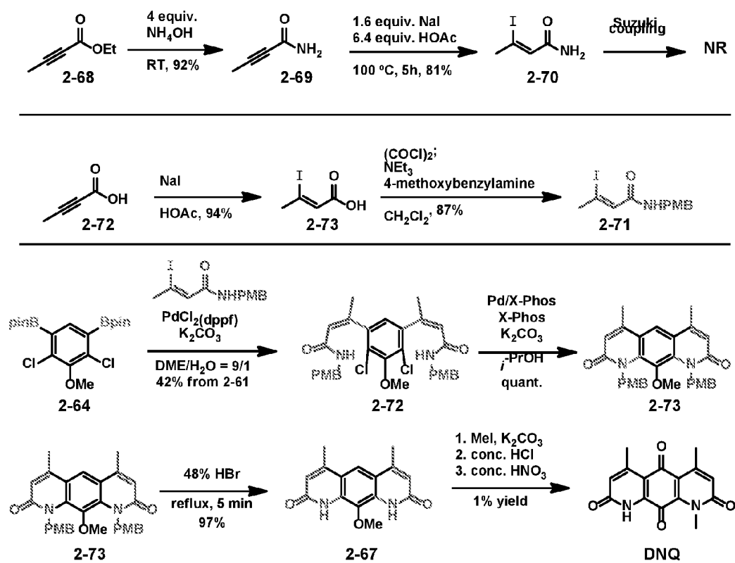
Scheme 1.13. Synthesis of DNQ by methylation of 2-67.
