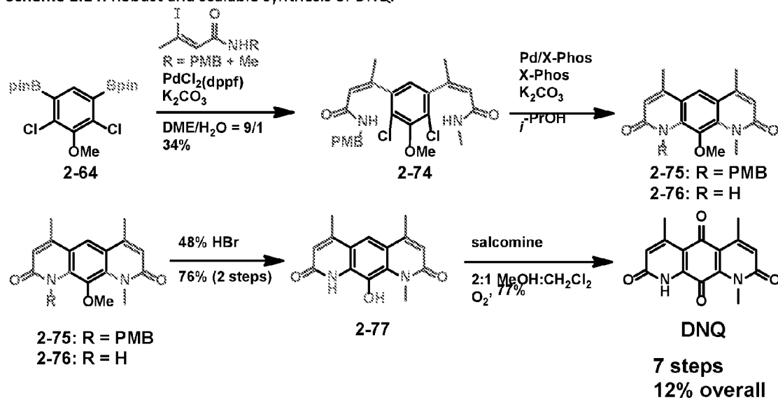
Scheme 1.14. Robust and scalable synthesis of DNQ.
