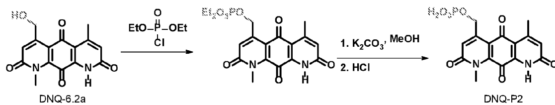
Scheme 7.3. Preparation of DNQ-P2 and DNQ-P3.
