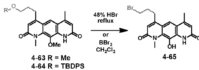
Scheme 4.6. Unexpected bromination of protected alcohols 4-63 and 4-64 during global deprotection.
