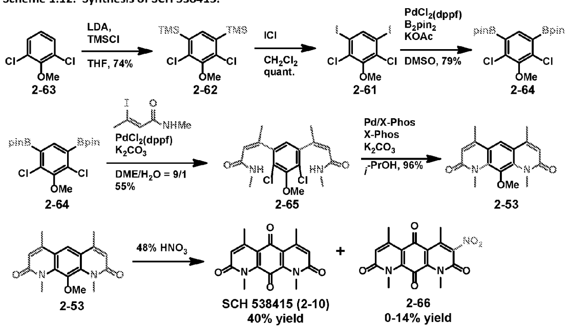
Scheme 1.12. Synthesis of SCH 538415.
