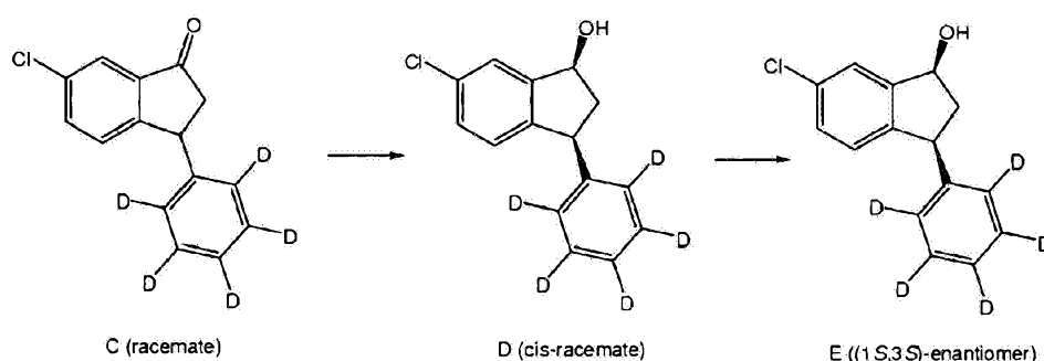
Scheme 10. Synthesis and resolution of Compound E.
