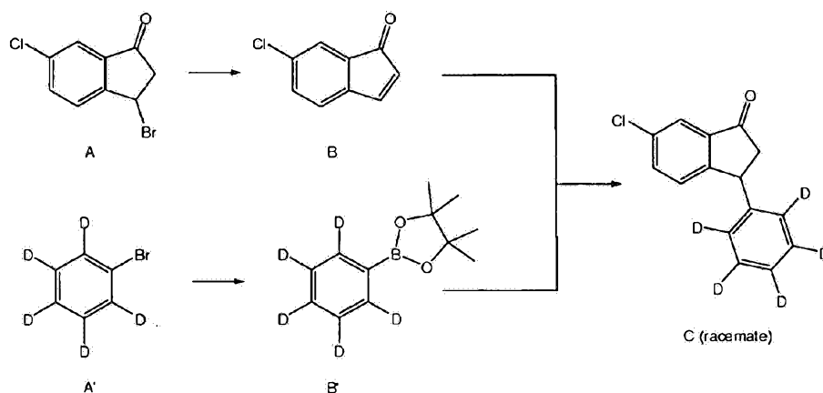
Scheme 9. Synthesis of Compound C.
