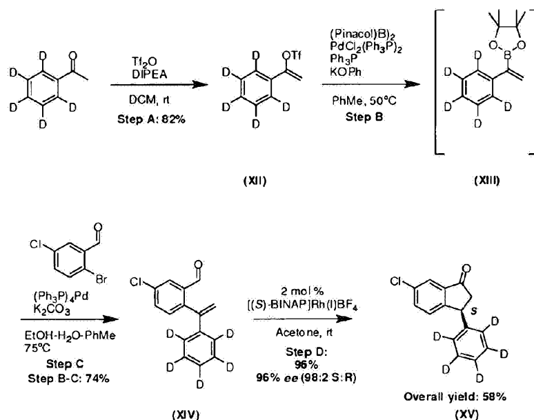
Scheme 14. Synthesis of Compound (XV)
