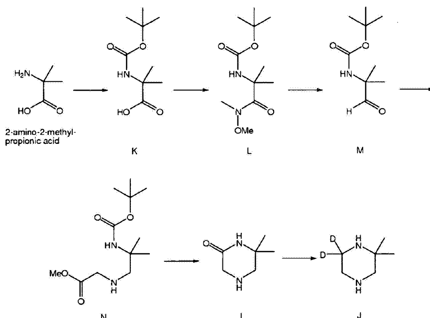
Scheme 7. Alternative exemplary synthesis of intermediate J.
