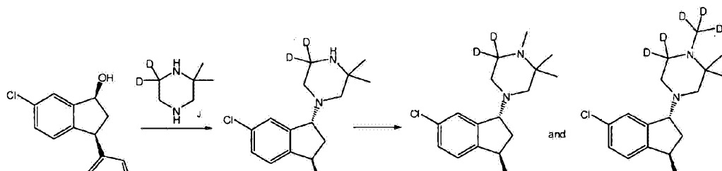
Scheme 12. Synthesis of Compound (III) and Compound (V).
