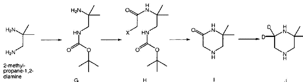
Scheme 6. Exemplary synthesis of intermediate J.
