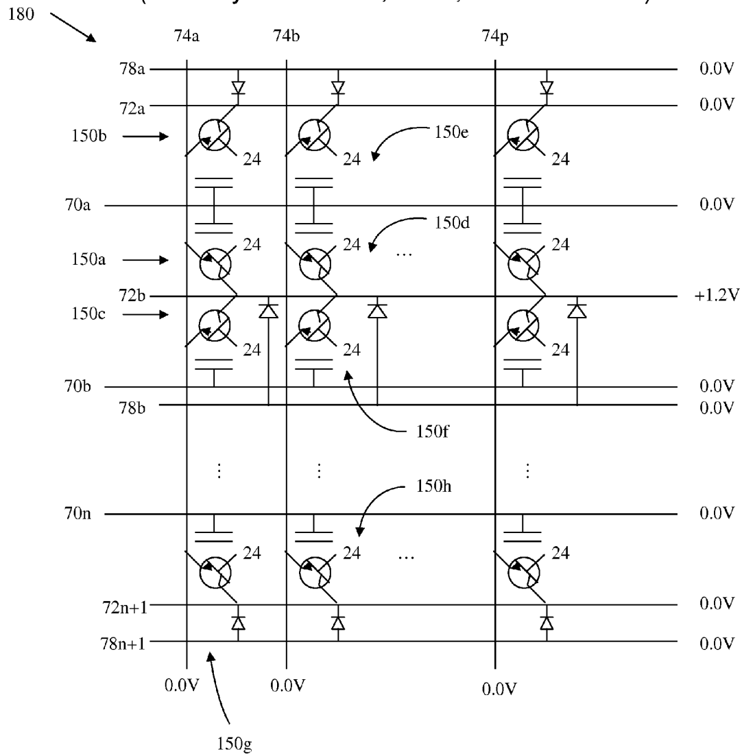
Two Row Hold Operation (Memory Cells 150a, 150c, 150d and 150f)
