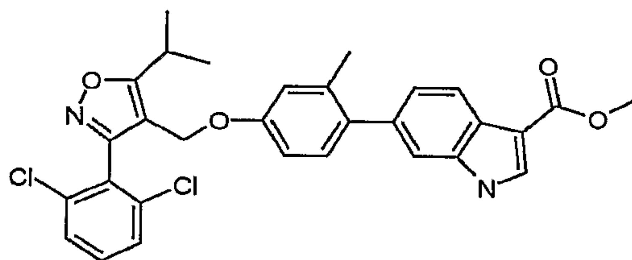
6-{4-[3-(2,6-Dichloro-phenyl)-5-isopropyl-isoxazol-4-ylmethoxy]-2-methyl-phenyl}-1H-indole-3-carboxylic acid methyl ester
