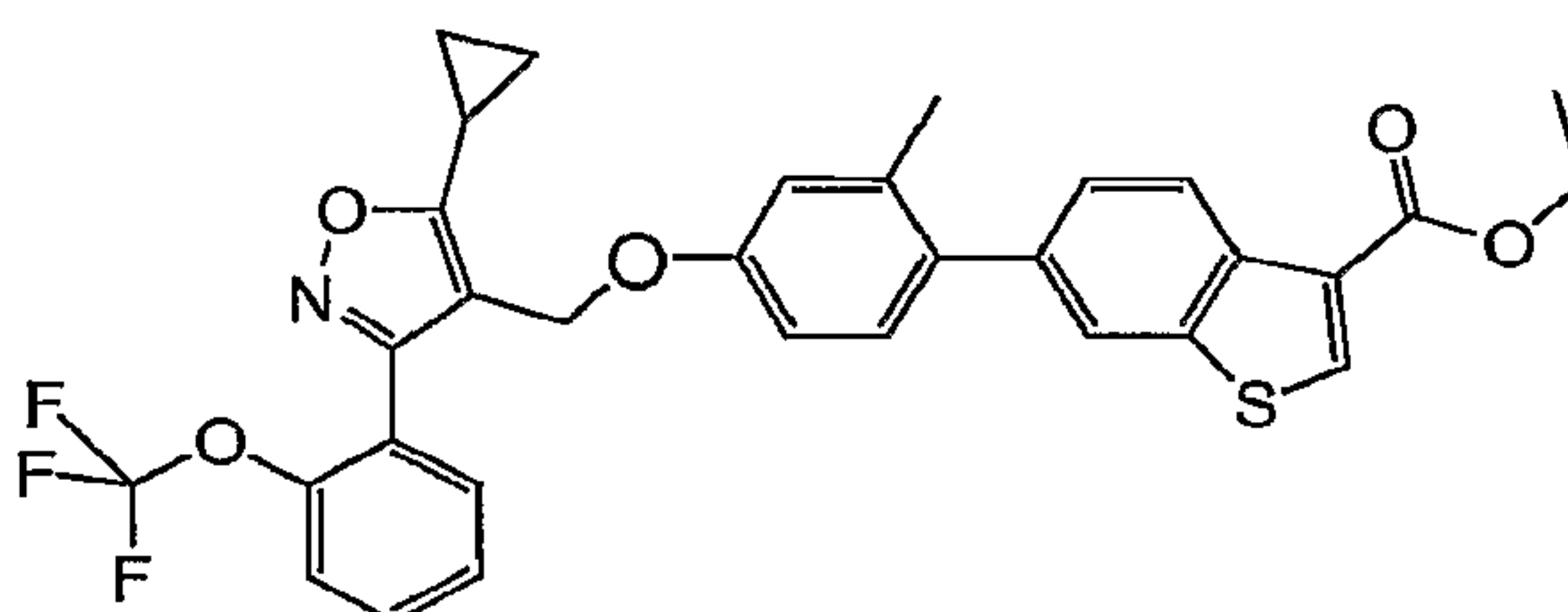
6-{4-[5-Cyclopropyl-3-(2-trifluoromethoxy-phenyl)-isoxazol-4-ylmethoxy]-2-methyl-phenyl}-benzo[b]thiophene-3-carboxylic acid ethyl ester
