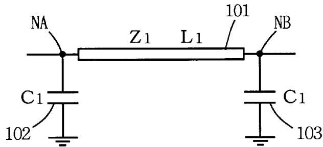
FIG. 38 PRIOR ART
