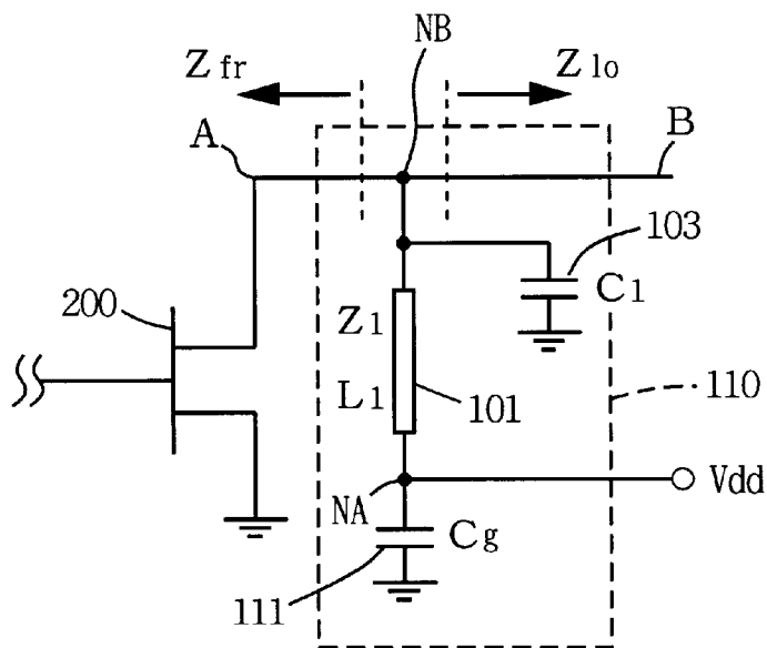
FIG. 39 PRIOR ART
