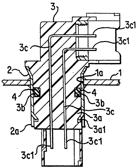
FIG. 18 PRIOR ART
