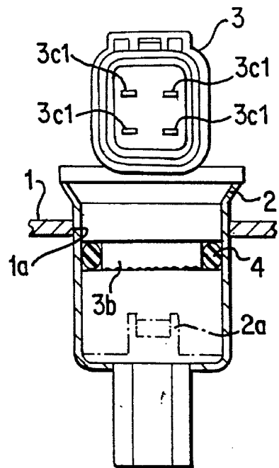
FIG. 19 PRIOR ART
