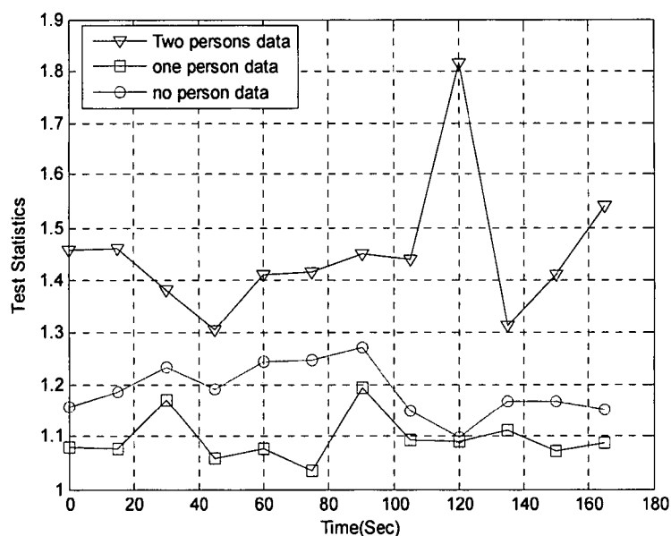
GLRT test for 2/1/0 person with 1 Ant
