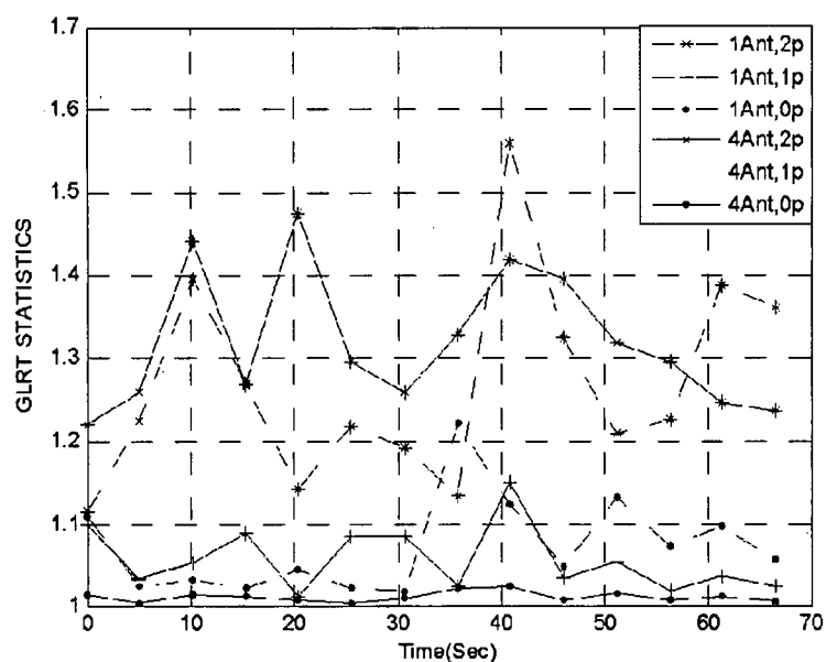
1 Ant versus 4 Ant GLRT test
