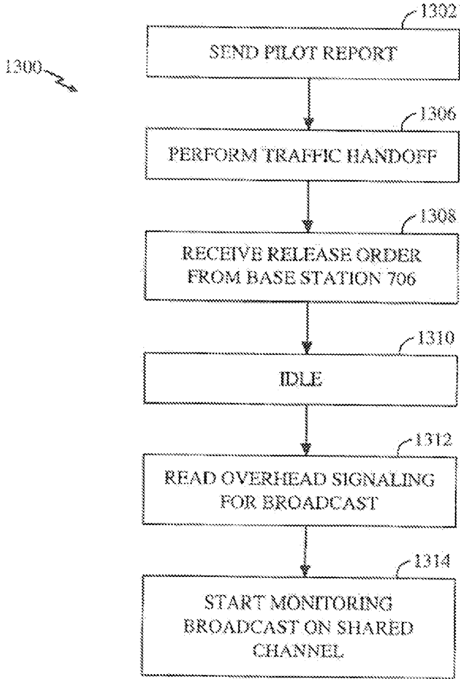
INDIVIDUAL-TO-SHARED HANDOFF OPERATION OF REMOTE (SECOND EMBODIMENT)
