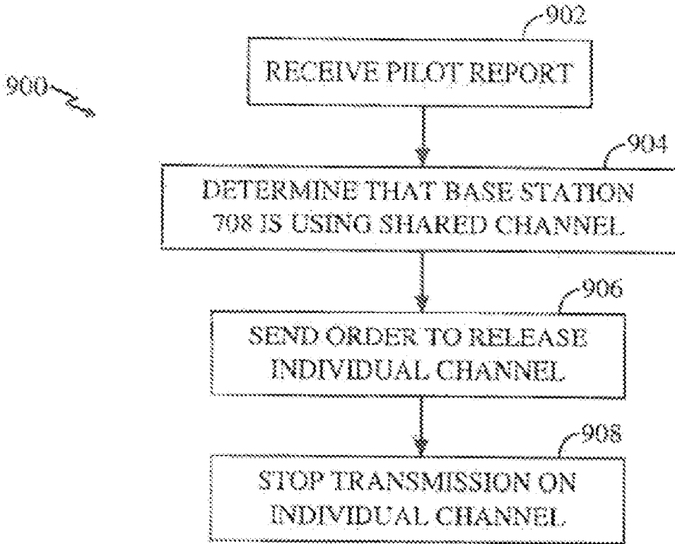
INDIVIDUAL-TO-SHARED HANDOFF OPERATION OF (INDIVIDUAL) BASE STATION (FIRST EMBODIMENT)
