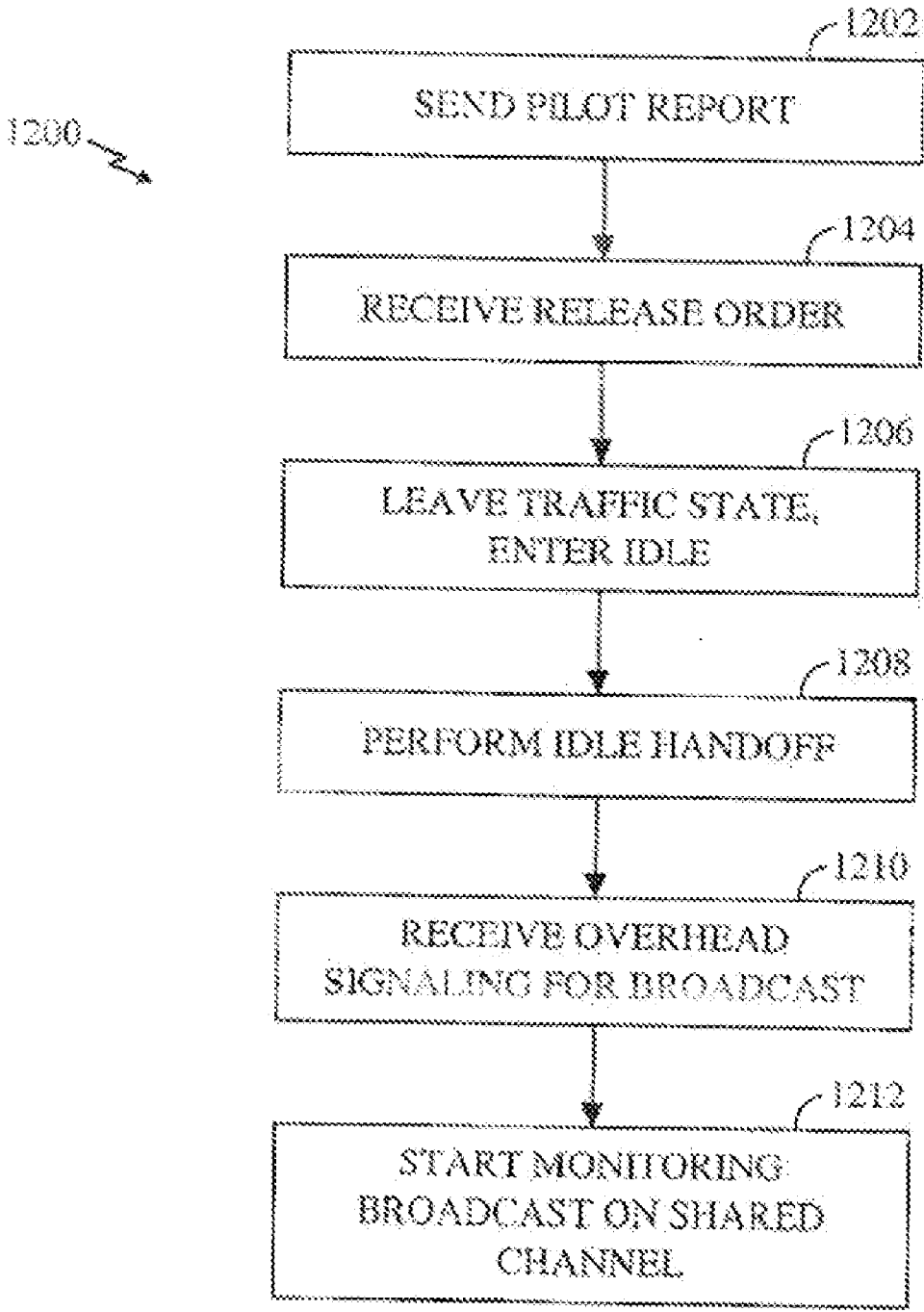
INDIVIDUAL-TO-SHARED HANDOFF OPERATION OF REMOTE (FIRST EMBODIMENT)
