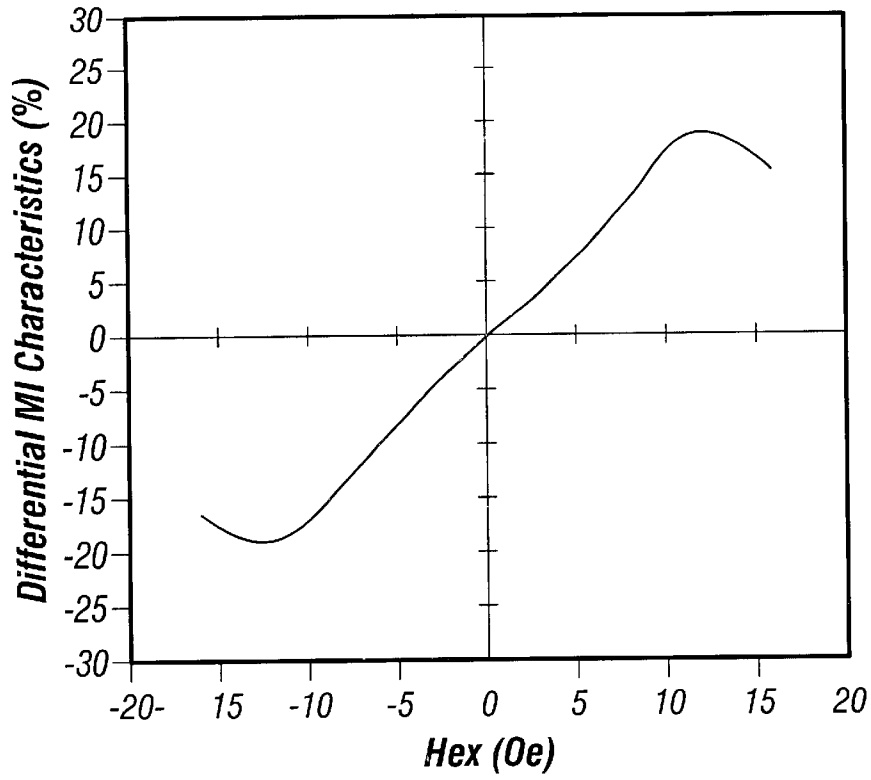
Hex (Oe) FIG. 10 (Prior Art)
